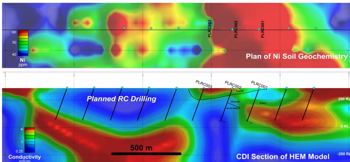
Figure 2. Actual and planned RC Holes over Image of Nickel Soil Geochemistry and HeliTEM Conductivity Depth Image (Cross Section 6434150N)
