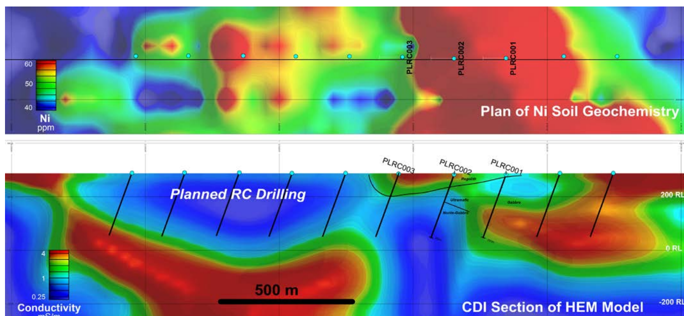
Figure 1. Actual and planned RC Holes over Image of Nickel Soil Geochemistry and HelITEM Conductivity Depth Image (Cross Section 6434150N)
