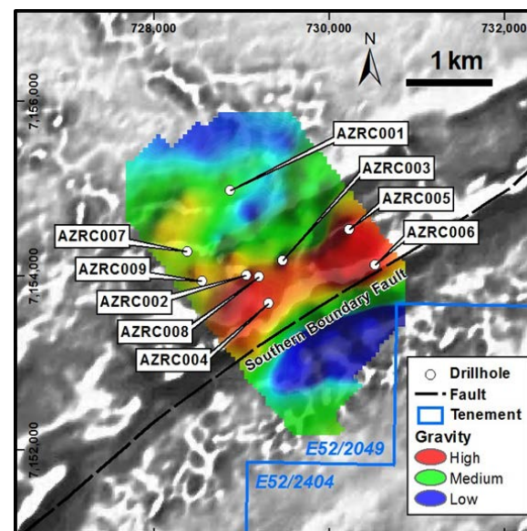
Bouguer Anomaly Gravity Image & RC Drill Holes
