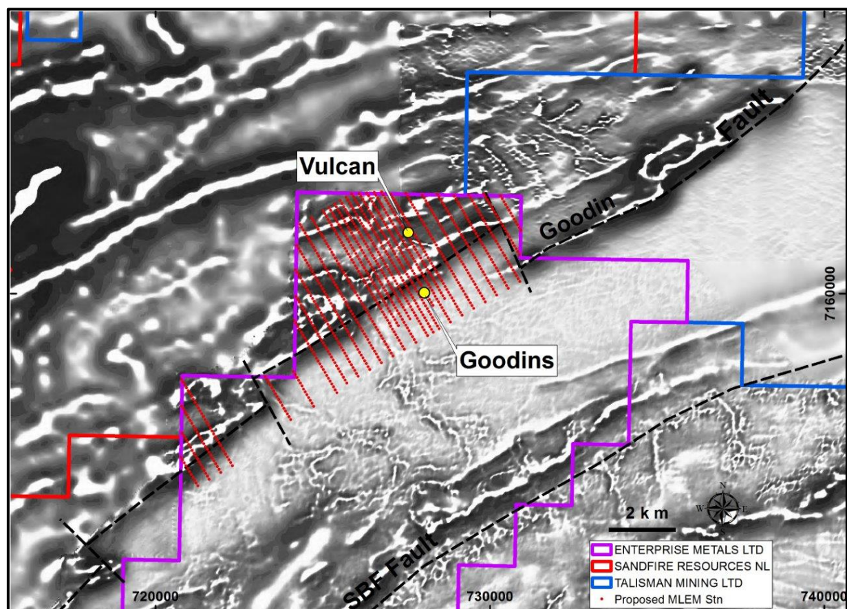
Figure 1. MLEM Lines (in red) over Magnetic Image and Geology Interpretation
