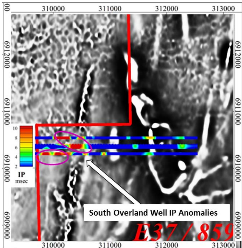
Figure 5. 2D IP Model 300m RL depth Slice on 1st VD Magnetic Image (IP targets in Magenta)
