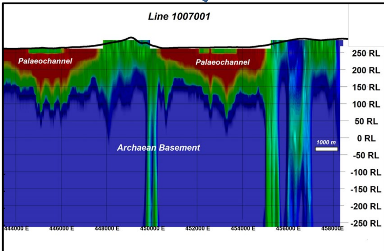
Figure 6. Sectional Model -
