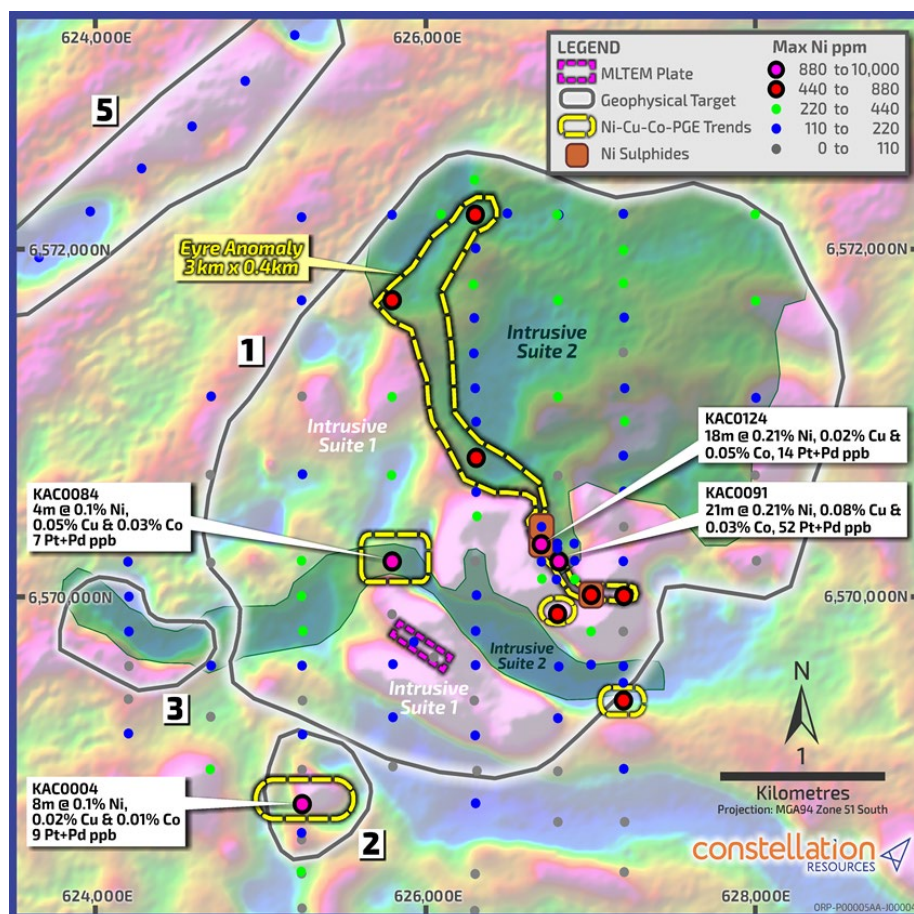
Figure 2. E28/2403 – Target 1 Intrusive &amp; Eyre Anomaly, Geochemical Footprints over 1VD Magnetic Image
