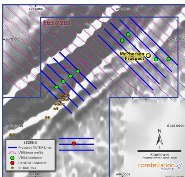
Figure 4. Proposed MLTEM Survey over VTEM and HelITEM Anomalies.
