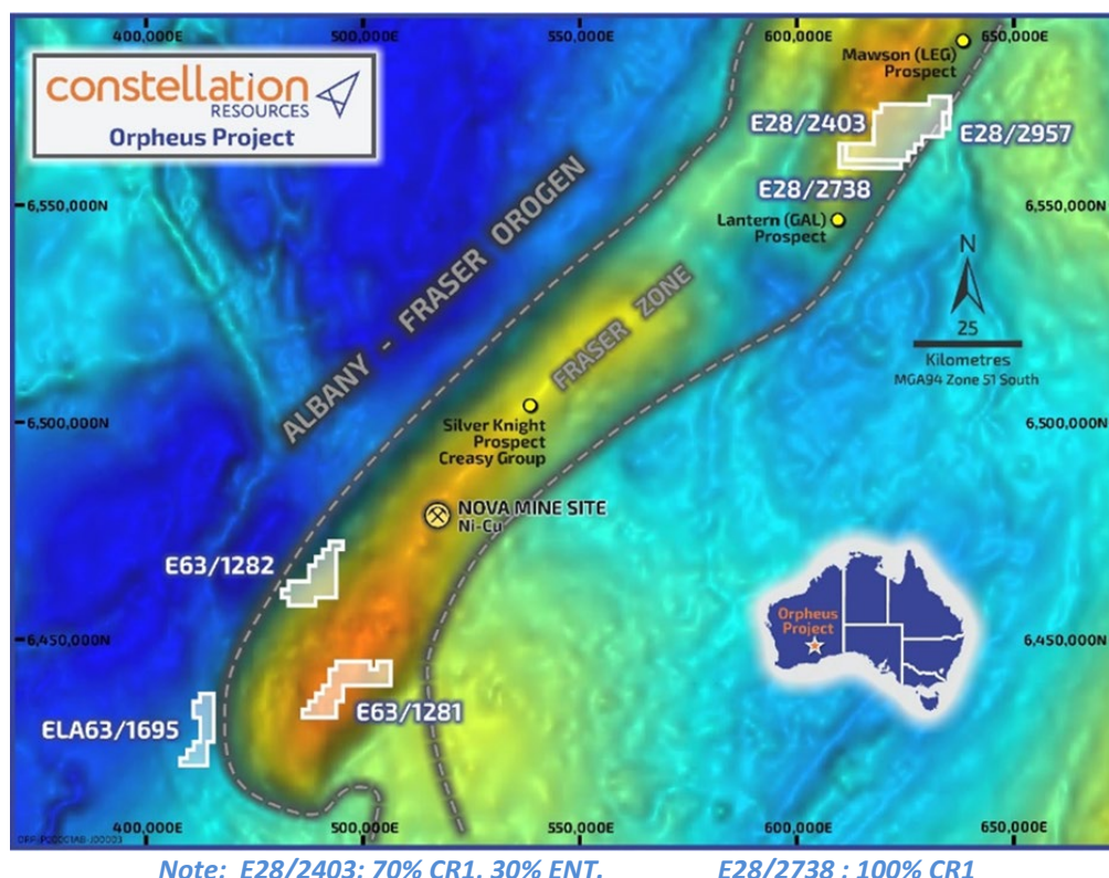
Figure 1. Location Plan, Orpheus Project Tenements.
