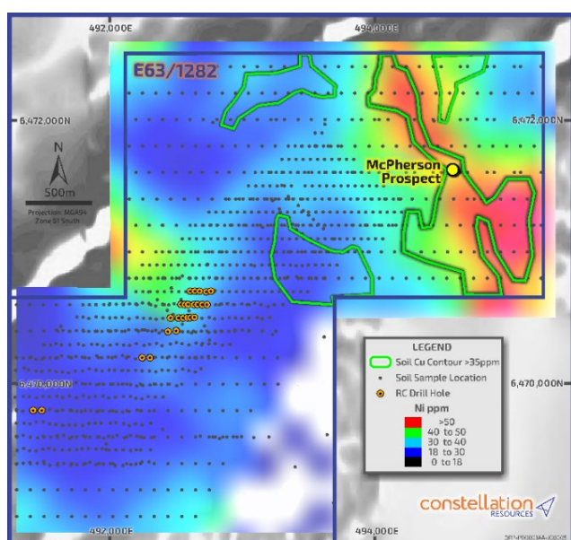
Figure 3. Ni-Cu Soil Geochemical Footprints over 1VD Grey Scale Aeromagnetic Image
