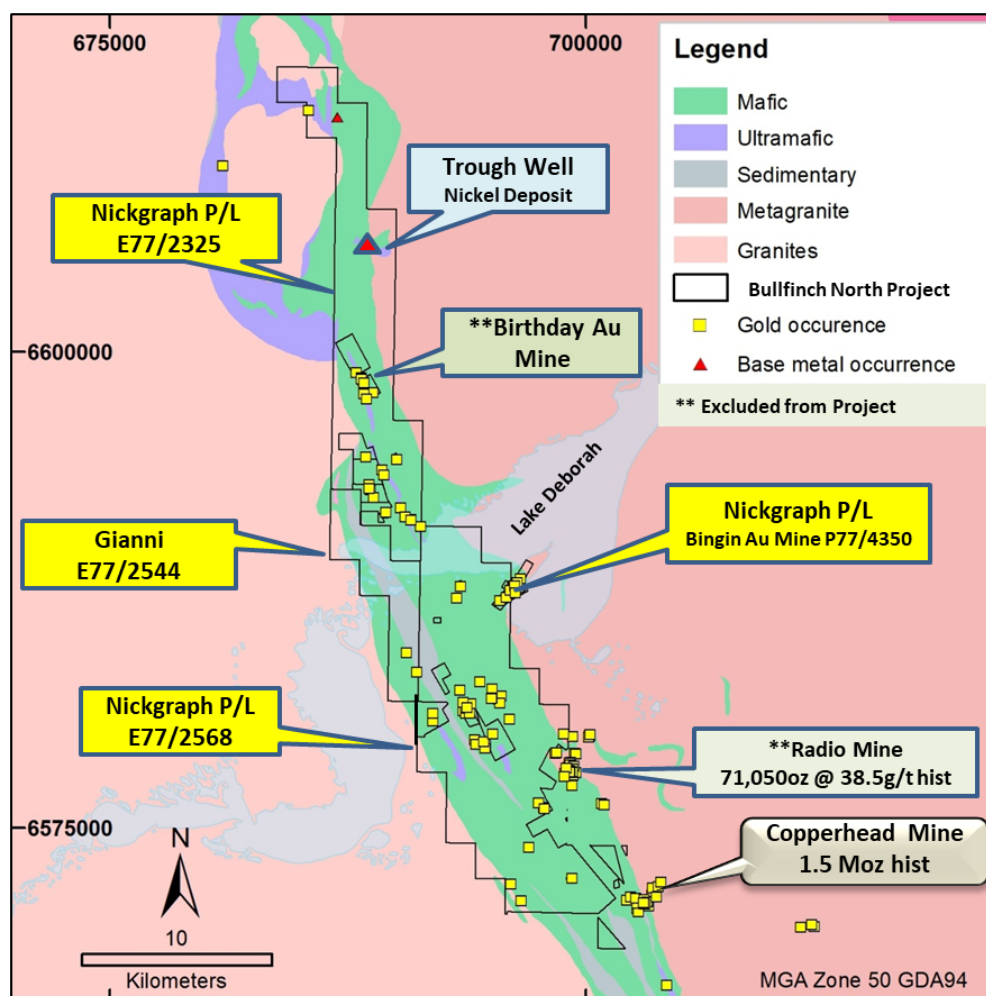
Figure 7. Bullfinch North Tenements Over Regional Geology
