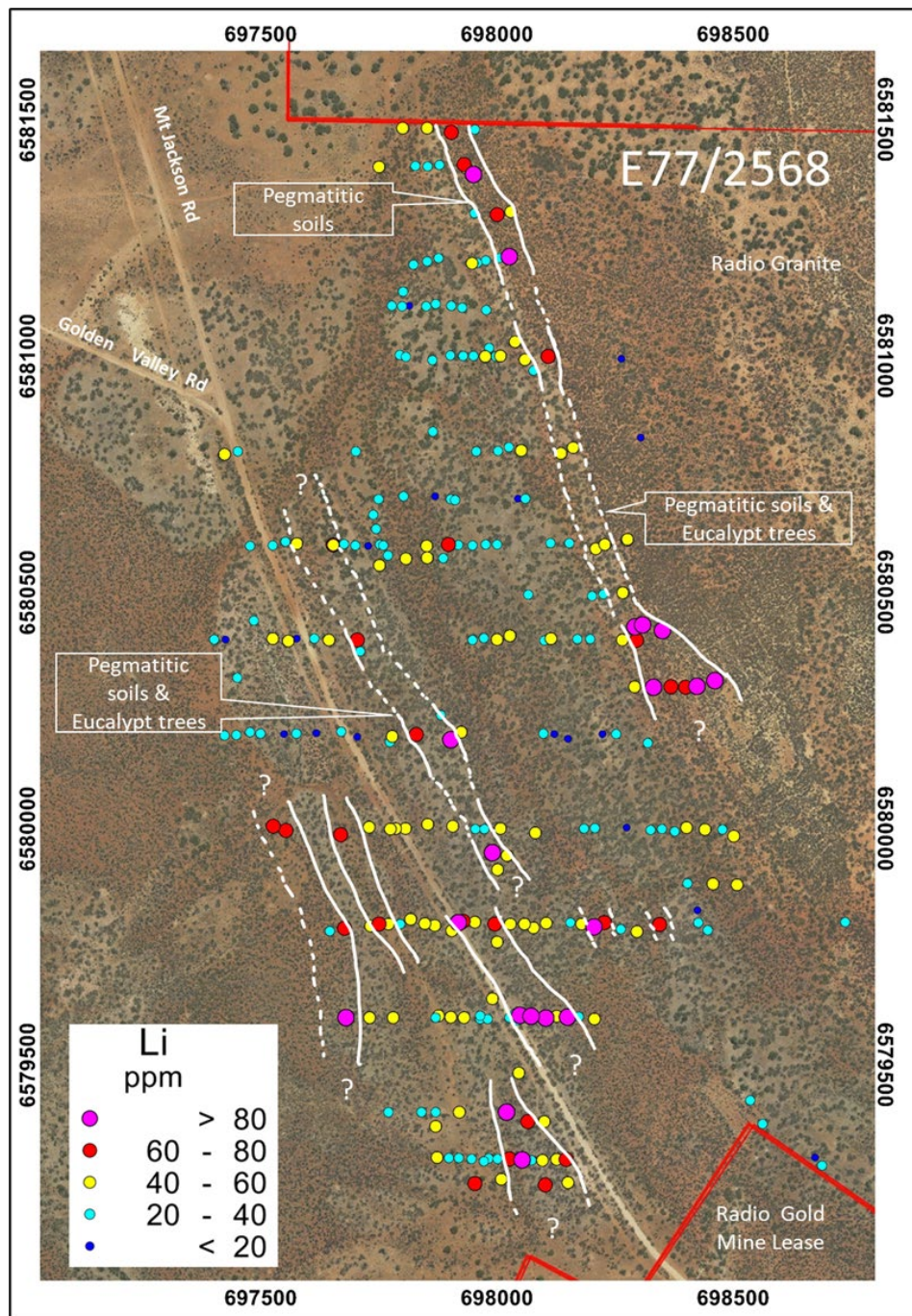
Figure 5. Image Showing Soil Sample Locations with Li ppm Assay Values
