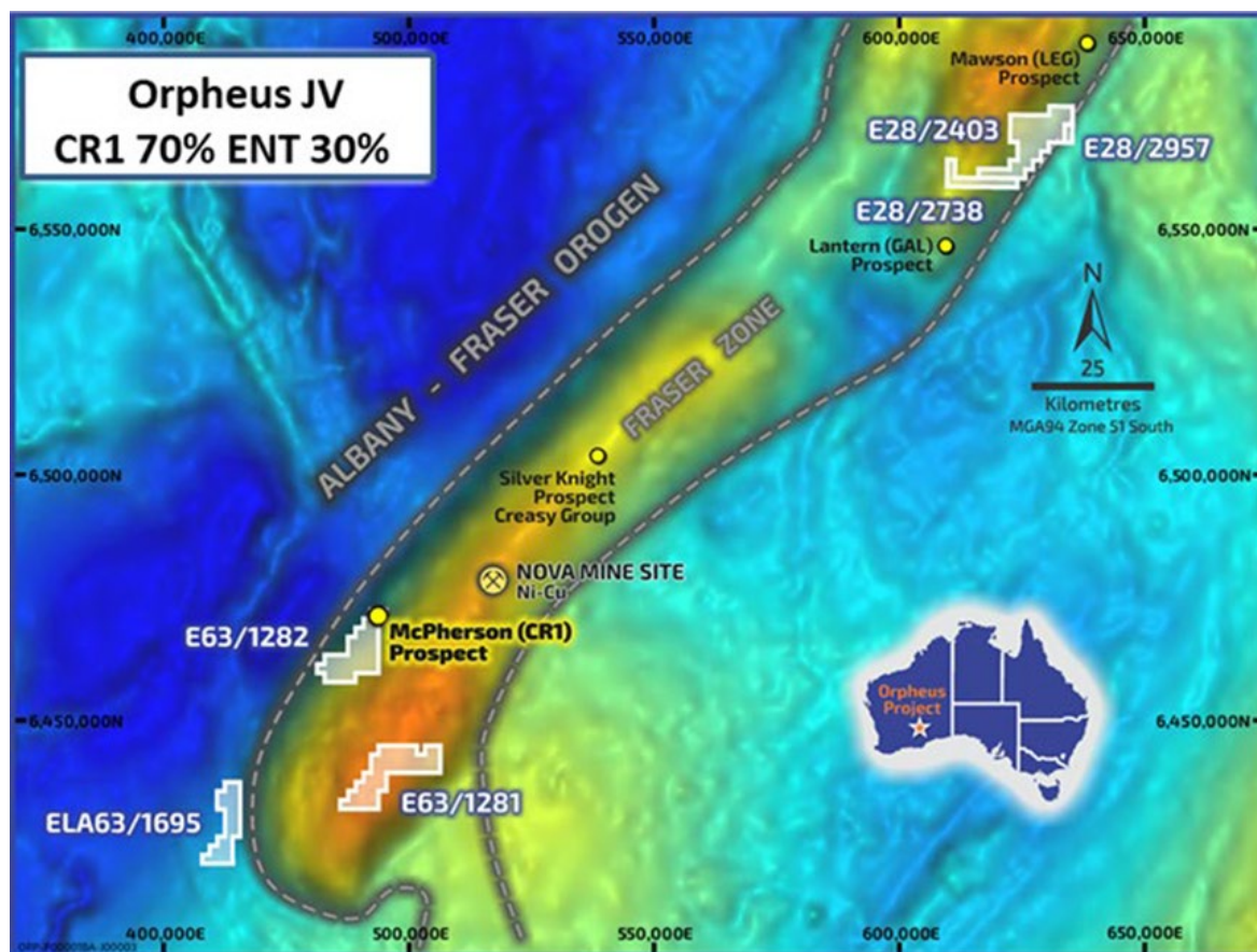
Figure 7. Location Plan, Orpheus Project Tenements E28/2403, E63/1281 & 1282 & ELA 63/1695.
