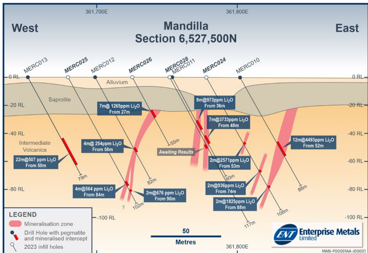
Figure 2. Mandilla Section 6527 600N – Pegmatite Interpretation & Lithium Oxide Intersections
