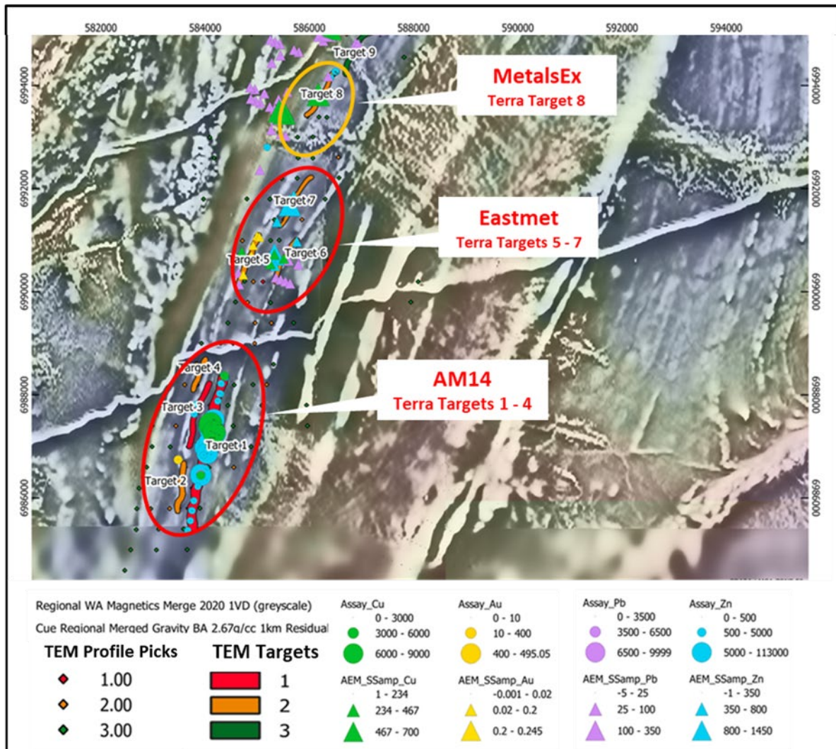
Figure 1. Priority Target areas on Conductivity Depth Image at 257RL over 1VD Magnetic Image
