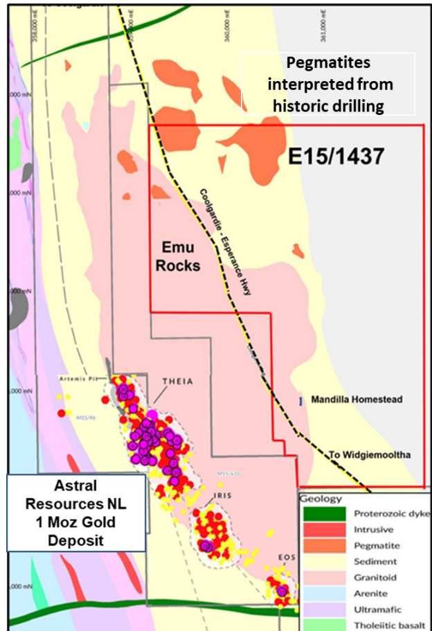
Figure 4. Geological Interpretation E15/1437
