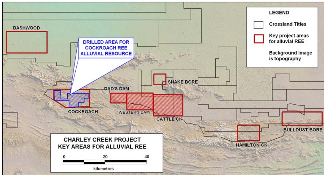
Figure 1 – Shows key areas for alluvial REE deposits
