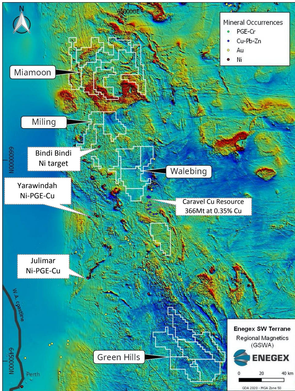
Figure 3 Enege project areas over regional airborne magnetics data
