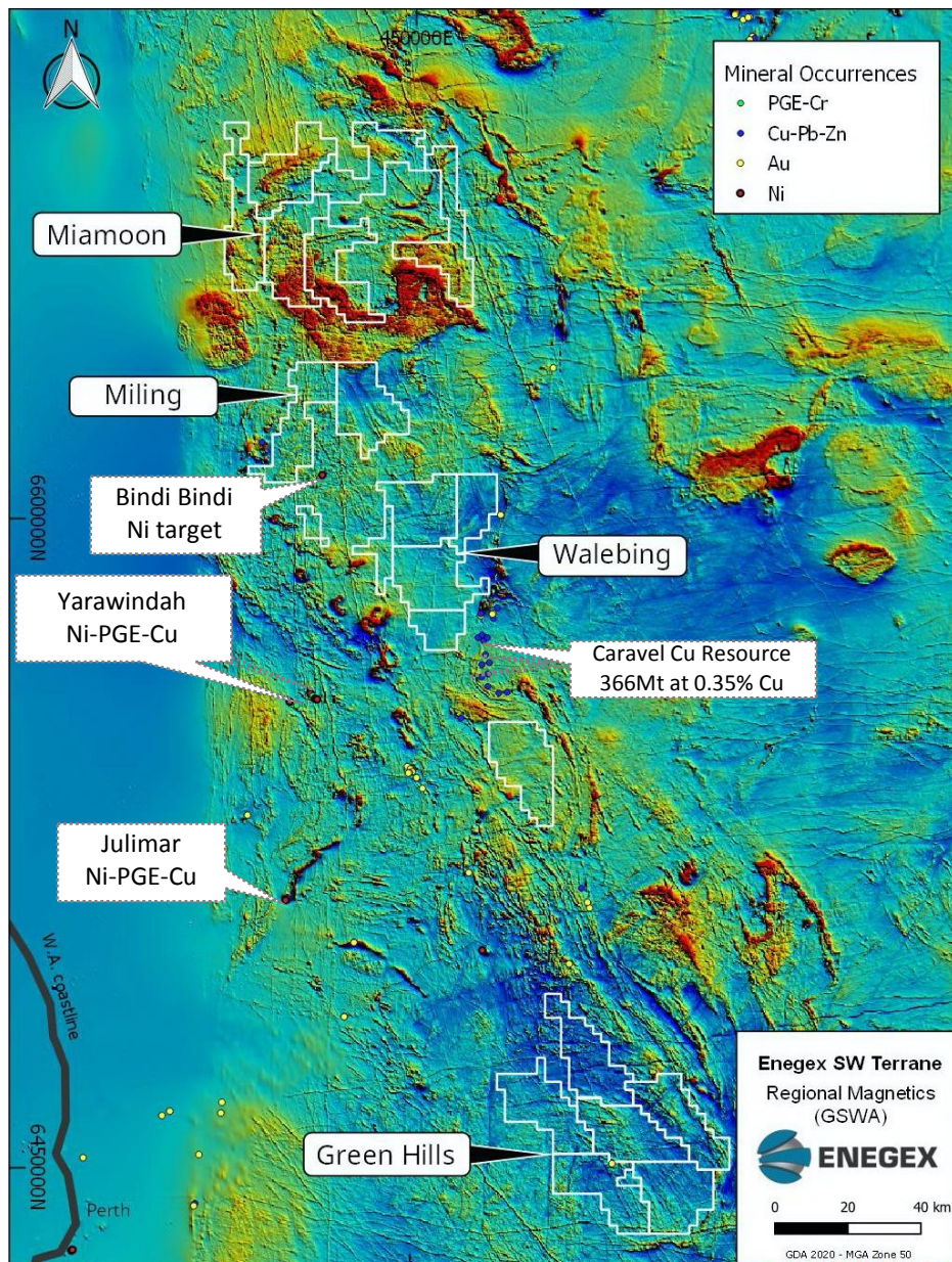
Figure 2 EnegeX project areas over regional airborne magnetics data
