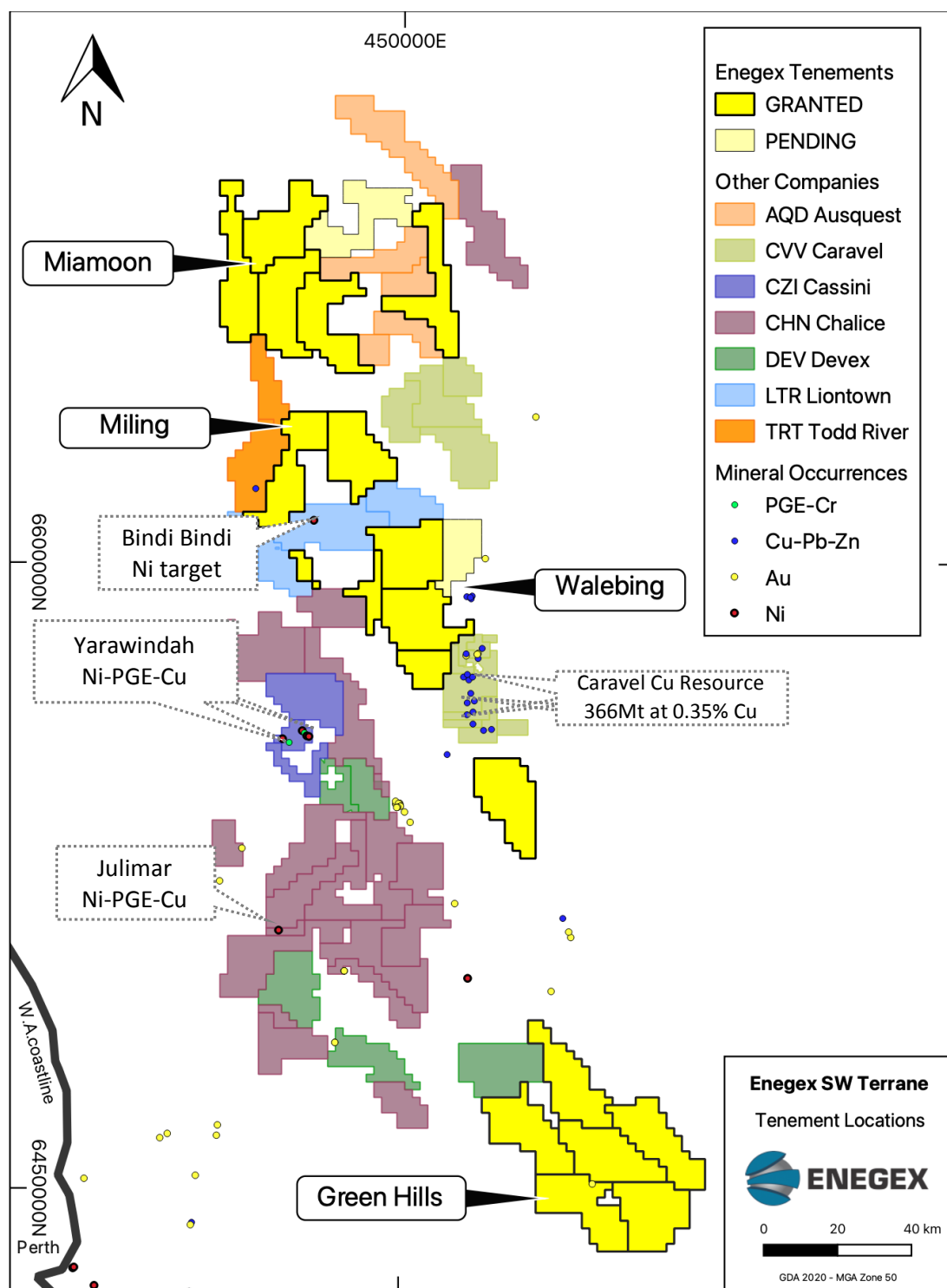
Figure 1 Enege South West Terrane Tenements
