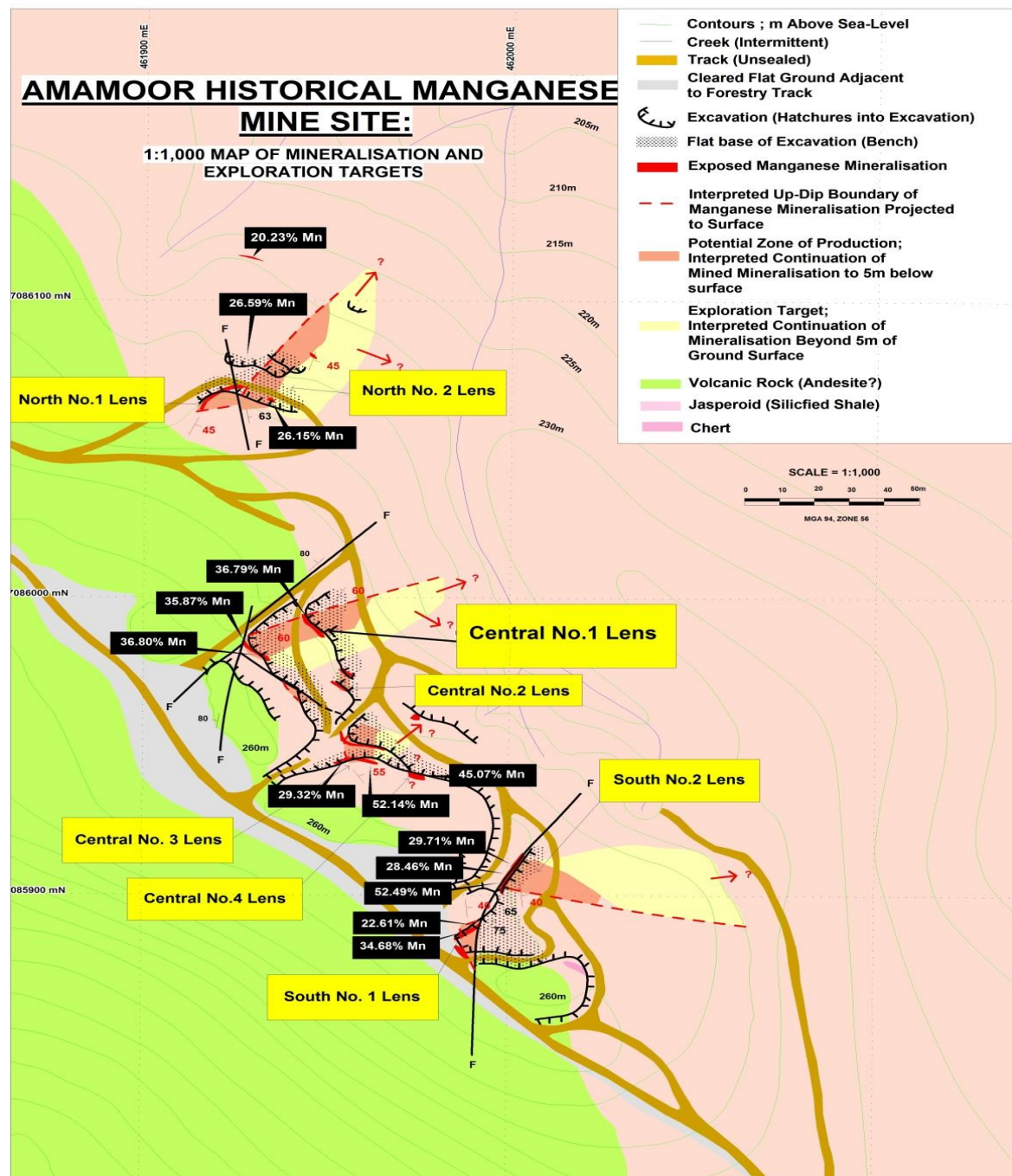
Figure 7. Amamoor Manganese workings
