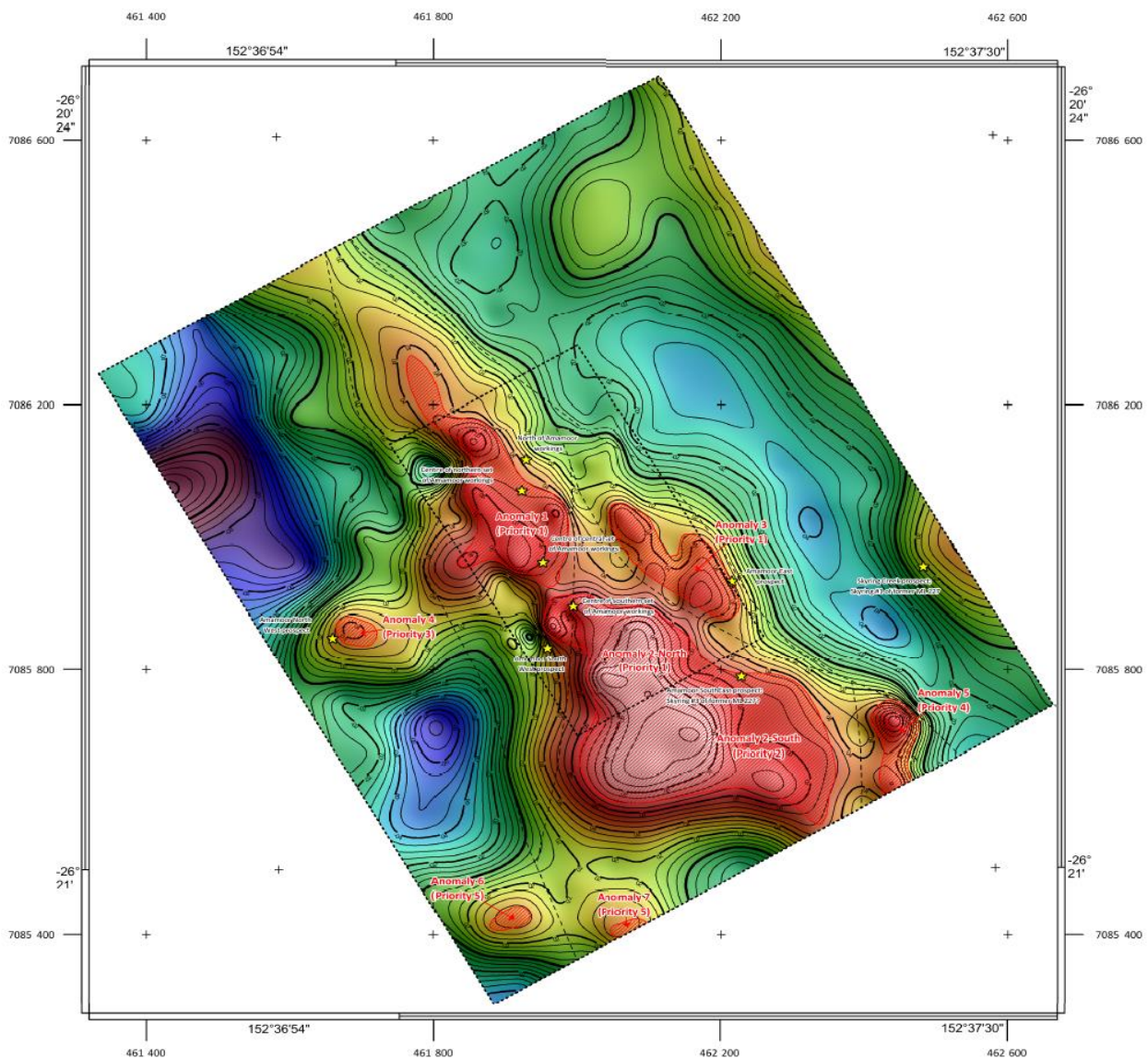
Figure 3: Amamoor Gravity anomaly map
