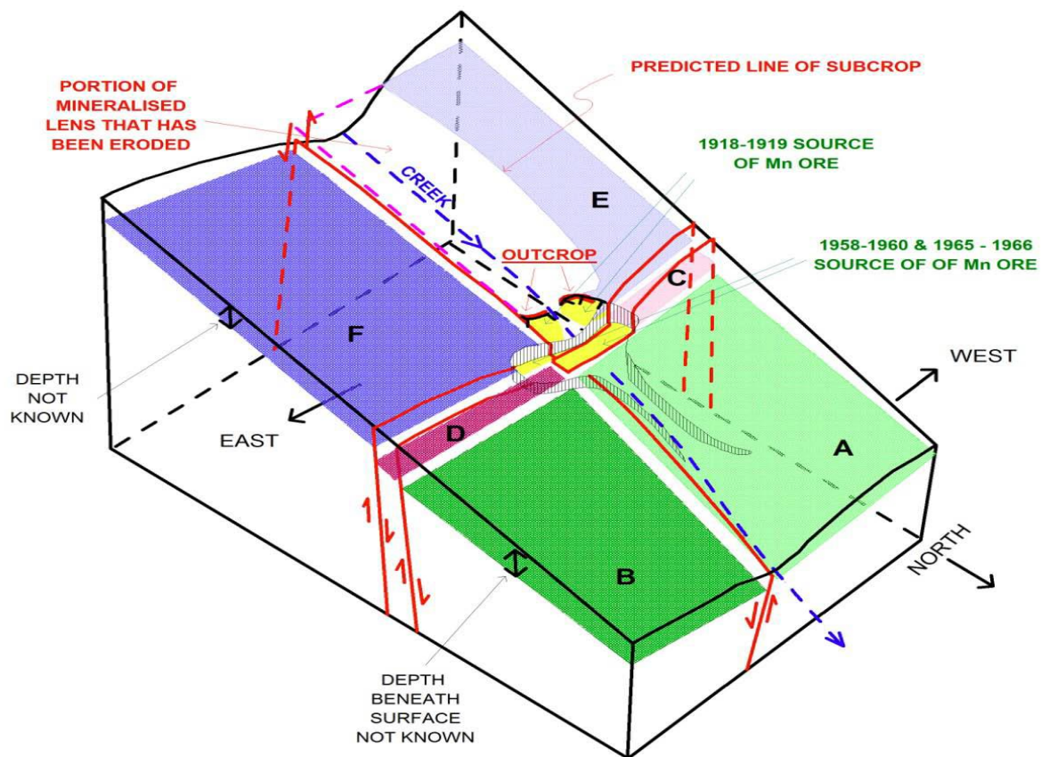
Figure 7: Theoretical 3-D Block model of mineralisation, Upper Kandanga Mn Mine
