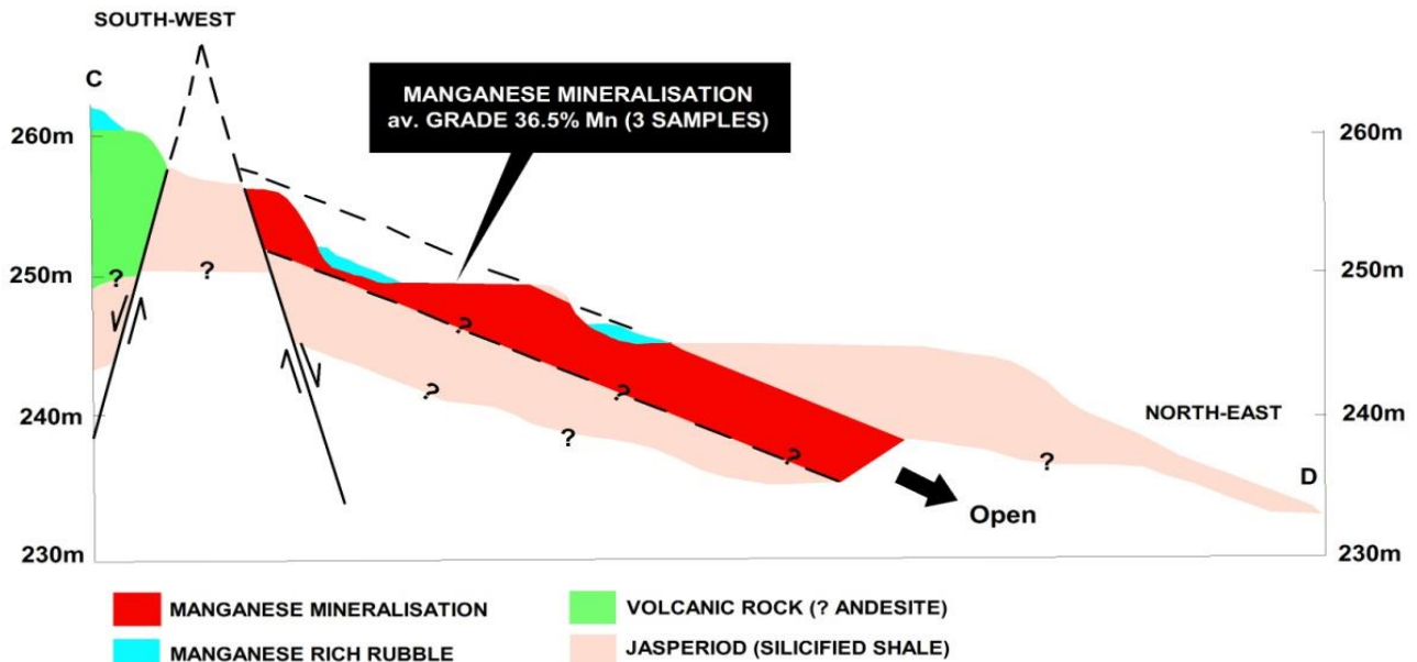
Figure 6. Amamoor cross section of Central Workings
