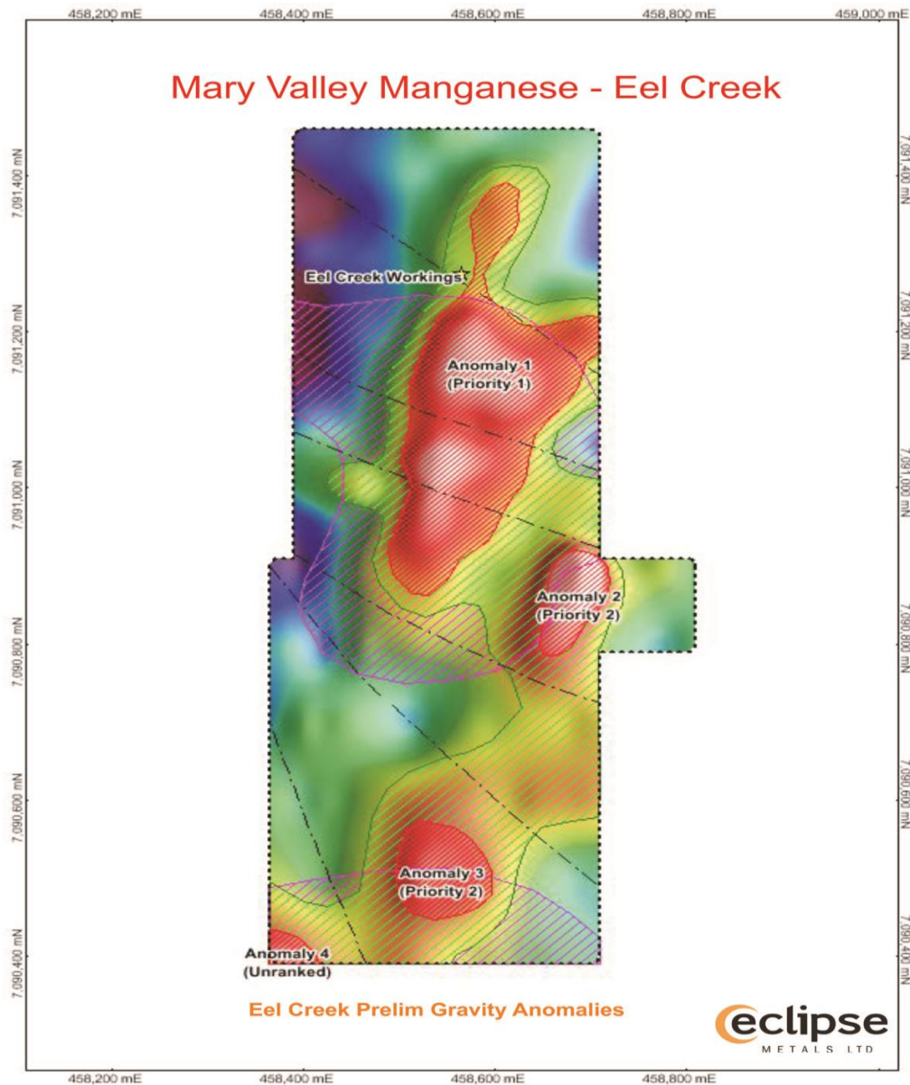
Figure 2 Eel Creek Preliminary Gravity anomaly map
