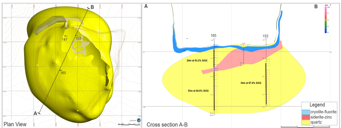
Figure 3: Plan view of the Ivigtut Pit showing Cross Section (A to B)
