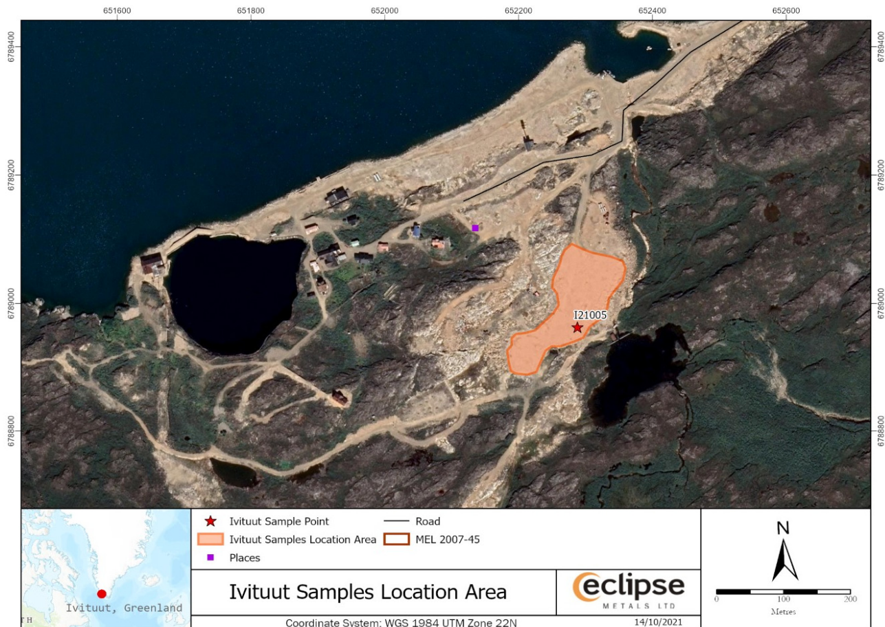
Figure 2: Image of the historic Ivigtut pit and waste dumps showing collection location for samples I21005
