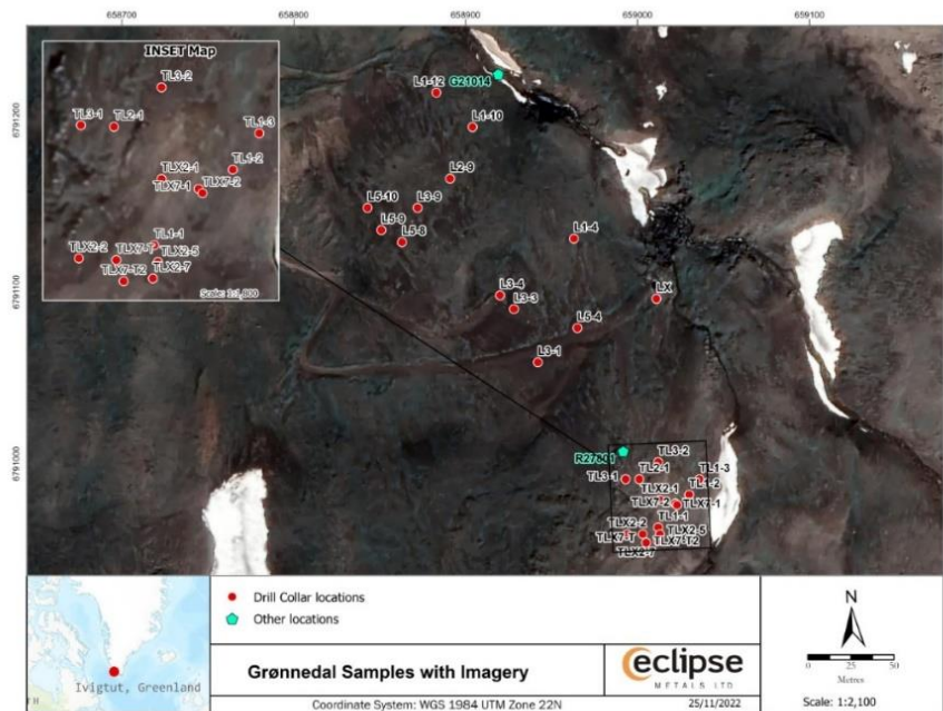
Figure 4: Grønnedal target area. Drill collars are marked with red dots while the two REE mineralisation styles are marked with green points. Assays are expected to be available toward the end of Q1-2023
