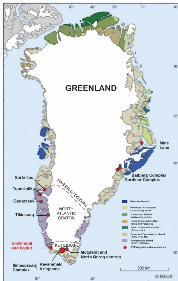
Figure 5. Greenland REE Deposits and location of Grønnedal and Ivigtut
