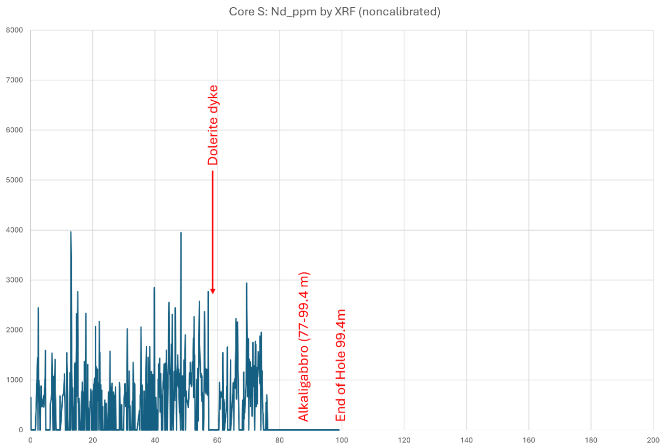
Figure 2: Nd (ppm) in Drillhole S, measured by the HyperXRF CS equipment, is uncalibrated (X-axis is depth; Y axis is Nd ppm)
