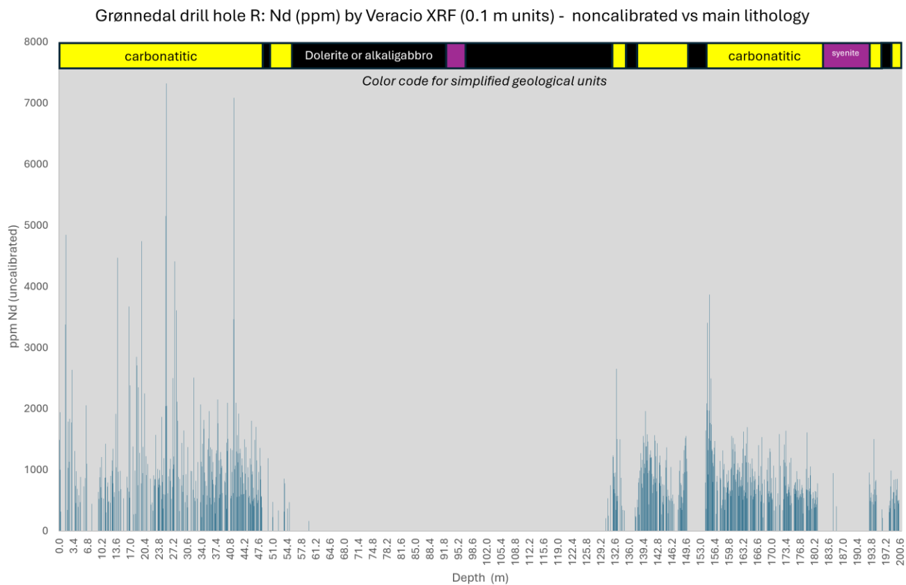
Figure 1: Nd (ppm) in Drillhole R, measured by the HyperXRF CS equipment, uncalibrated (X-axis is depth; Y axis is Nd ppm)
