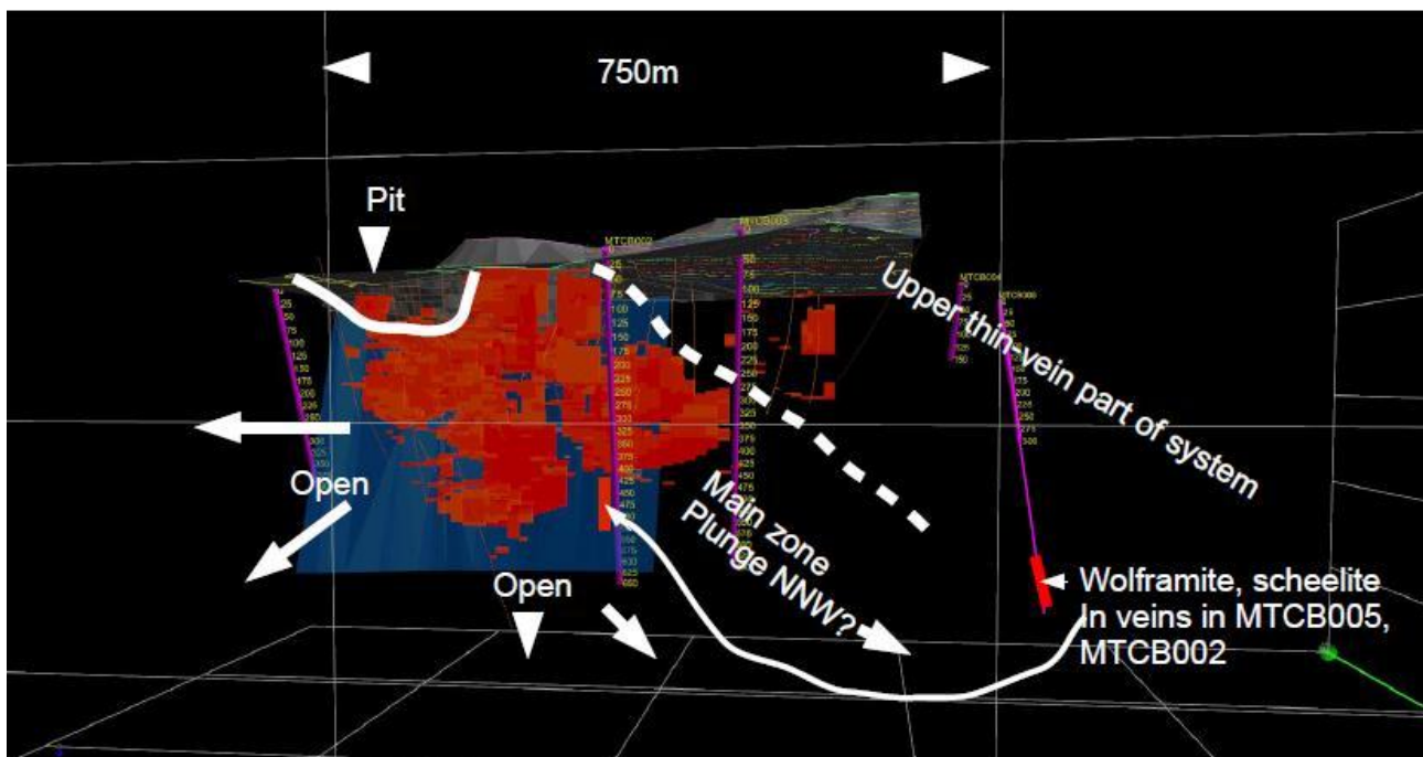
Figure 3. Cross section looking west, showing >0.14% WO 3 mineralisation (red), and location of sheeted quartz vein-hosted tungsten mineralisation encountered in drill holes MTCB 002 and 005, (projected to plane of the cross section), and indications of where mineralisation is open (untested by drilling).
