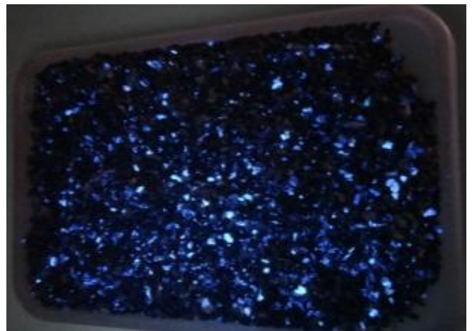
Coarse -3mm jig concentrate under UV light show that the scheelite is present as liberated grains.
