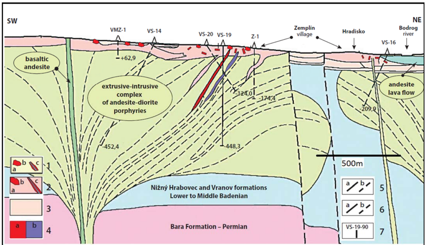
Cross section through the Zemplin structure. Prospech will seek to repeat the silver mineralisation intersected in VS19 and 20, down dip and along strike.
