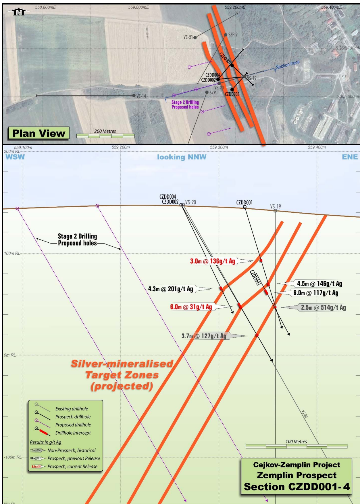
Cross section through the Zemplin series of parallel silver-bearing structures. Additional drilling planned to follow extend down dip and along strike.
