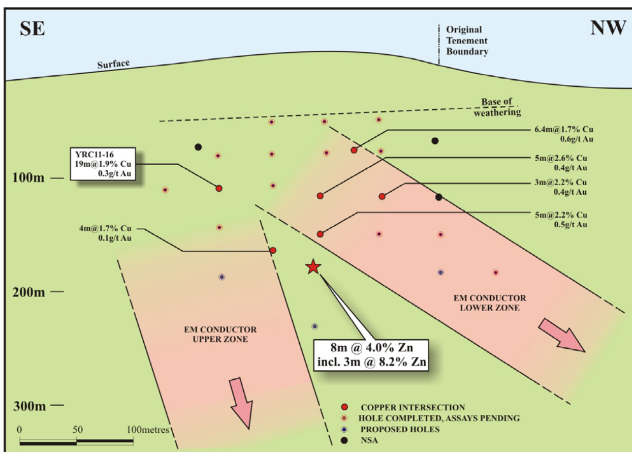
Figure 3: A Zone Long Section
