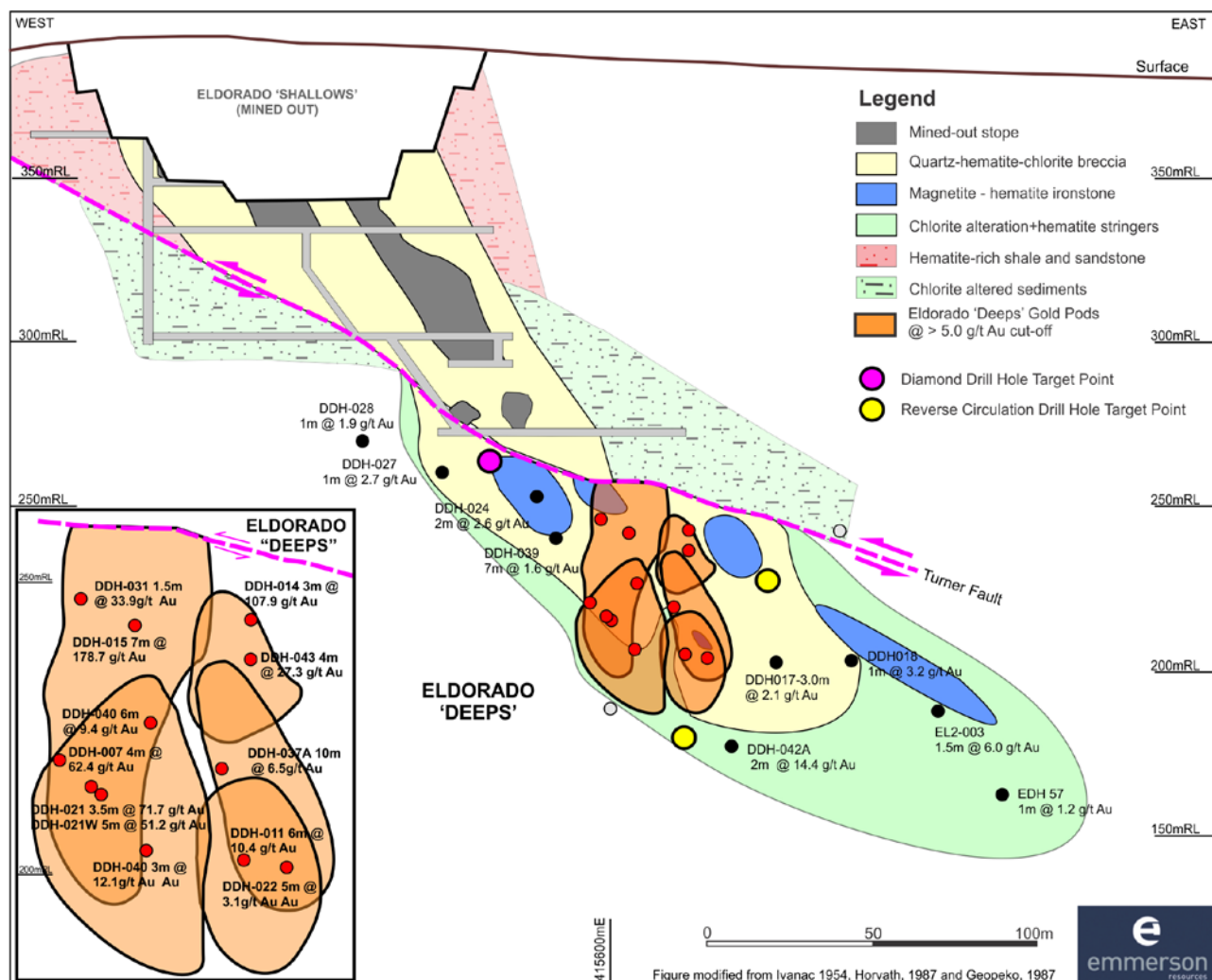
Figure 2 – Eldorado long section showing the mineralization, alteration, historic grade and the location of proposed drill holes (pink and yellow) to test the un-mined extensions.
