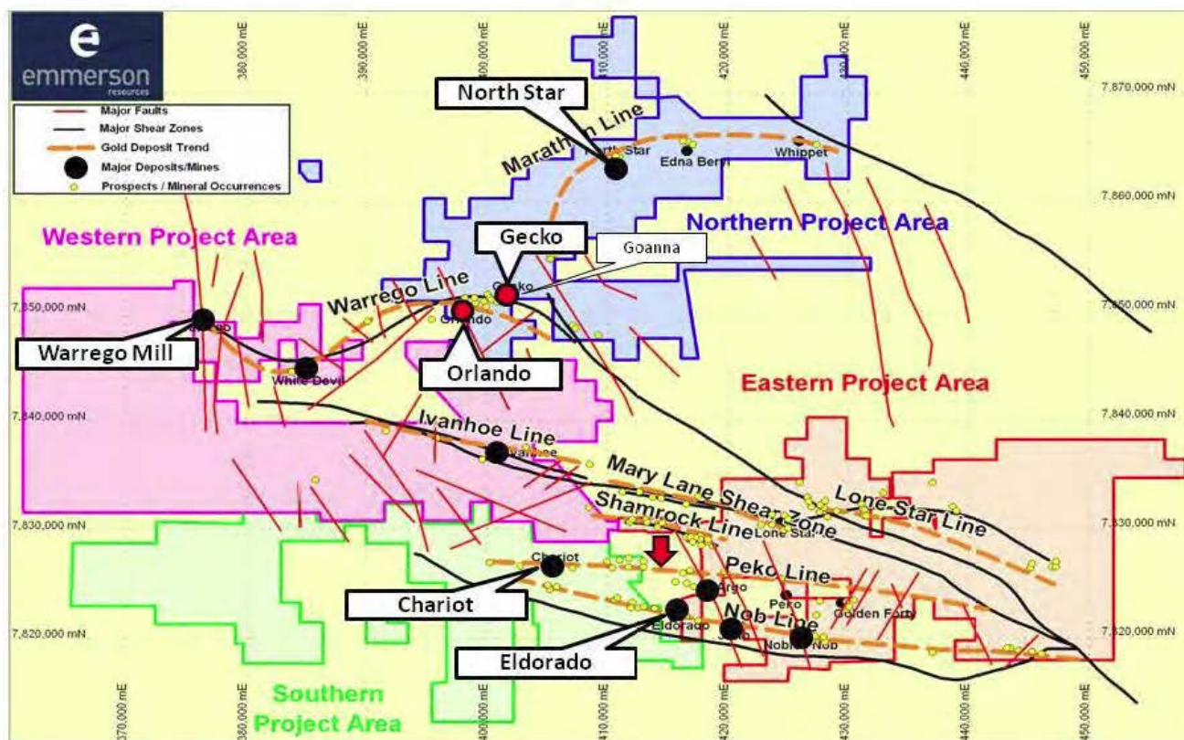
Figure 1 – location diagram of Chariot and Eldorado, showing major trends and structures
