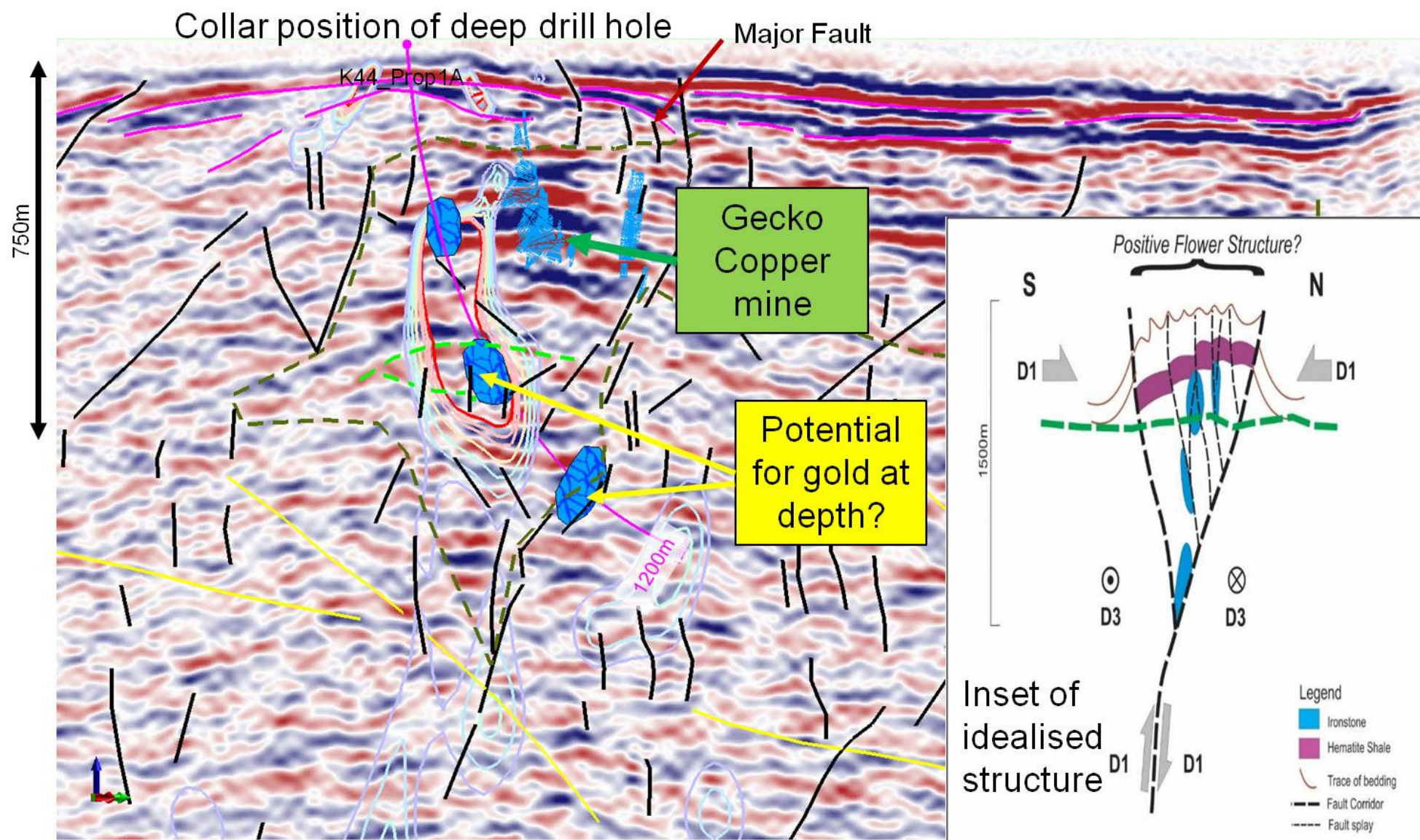
Figure 2: Trace of deep drill hole (purple) on background of seismic reflection. Metal zonation of near surface copper to gold at depth (based on historic mines in the TCMF)
