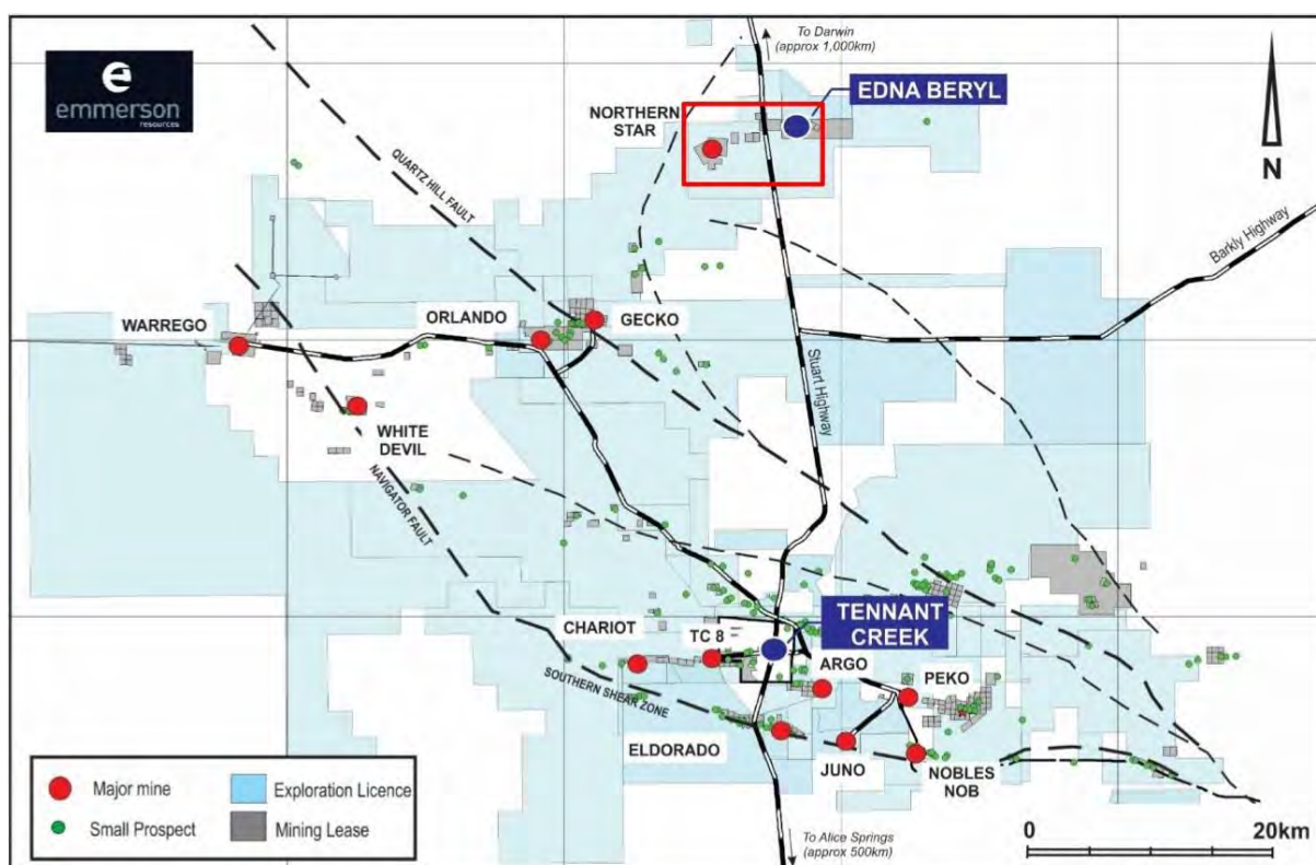
Figure 1: Emmerson's Tennant Creek project area
