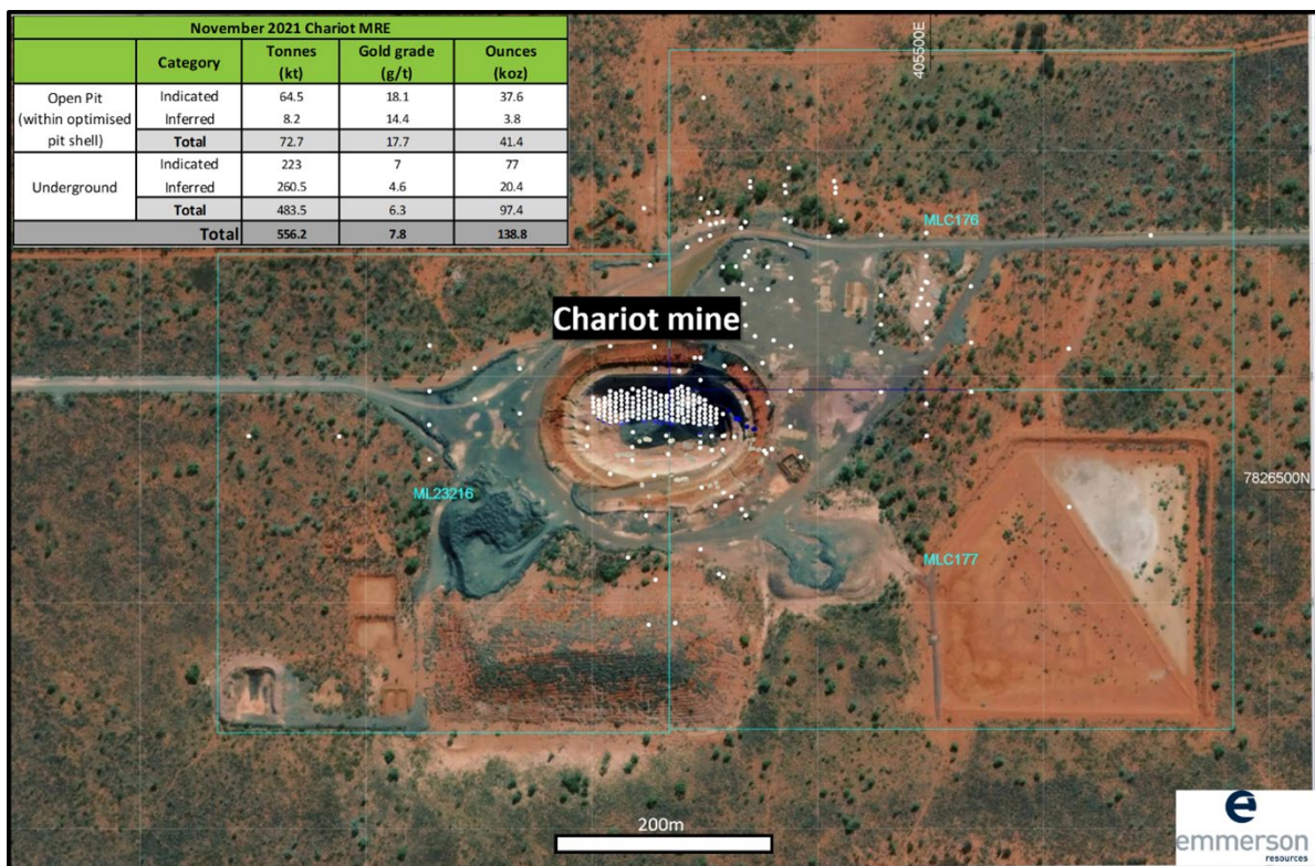
Figure 2: Plan view of Chariot Deposit and drill hole location. Also showing the Chariot Mineral Resource Estimate.
