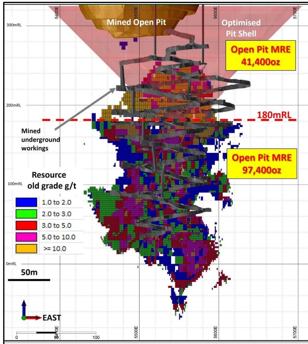
Figure 3: Chariot Mineral Resource Estimate - gold grades above 1g/t, not mined (looking North).
