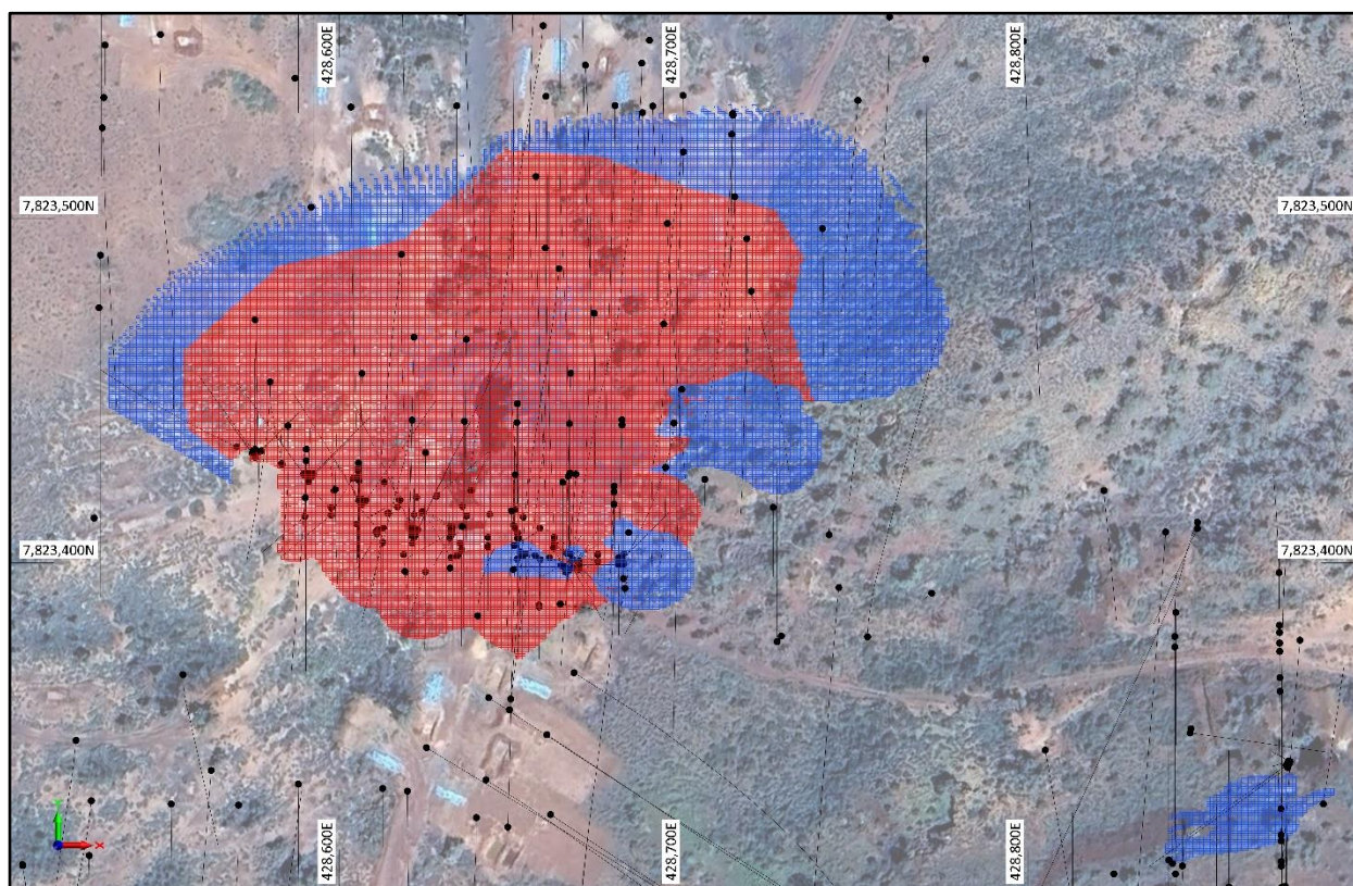
Figure 2: Golden Forty Drill Hole Collar Plan with block model coloured by Resource classification (Red Indicated, Blue Inferred).
