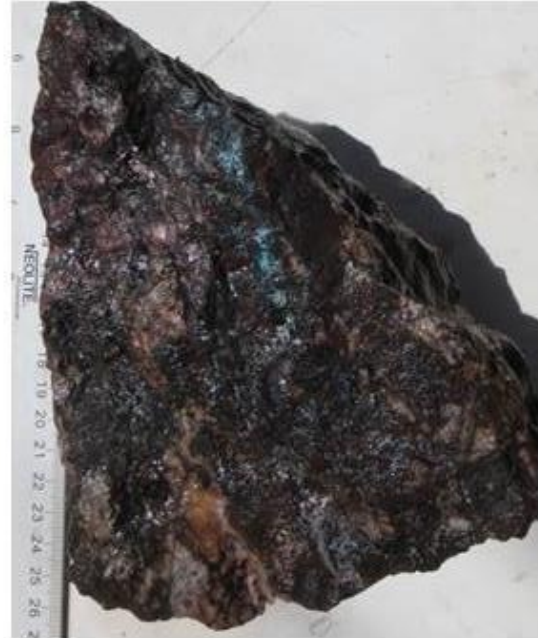
A. Argillic dacite breccia with caliche-red haematite matrix and quartz-partially leached sulphides-, atacamite (Cu-Ox) in veinlets and cumulus. Subcrop. (406187E 7499057N PSAD56 19S)
