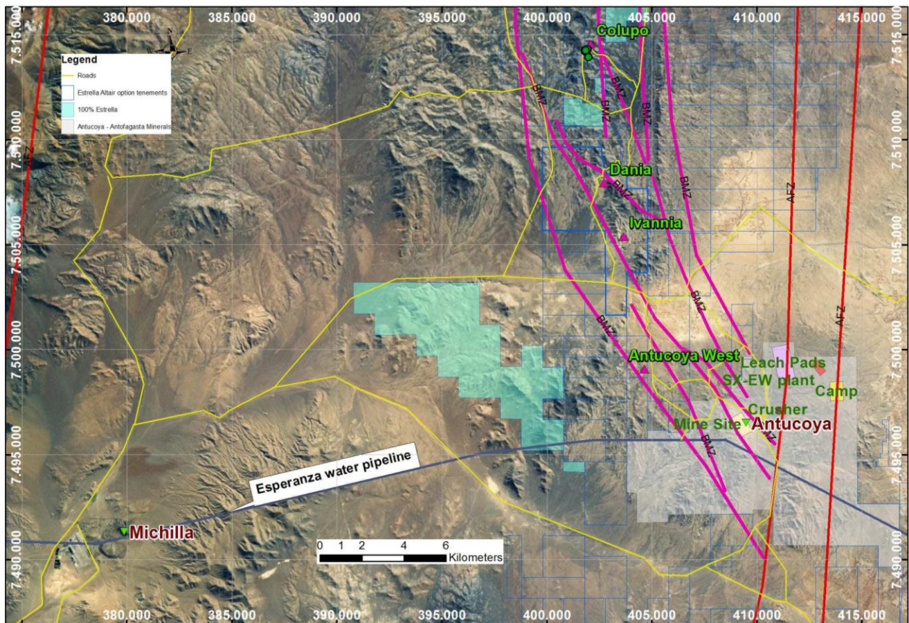
Figure 2: Antofagasta Minerals' Michilla and Antucoya mines locations in relation to Estrella's current drilling program at Antucoya West. Estrella is focussed on the mapped occurrences of copper mineralisation within the Buey Muerto Fault Zone (BMZ).
