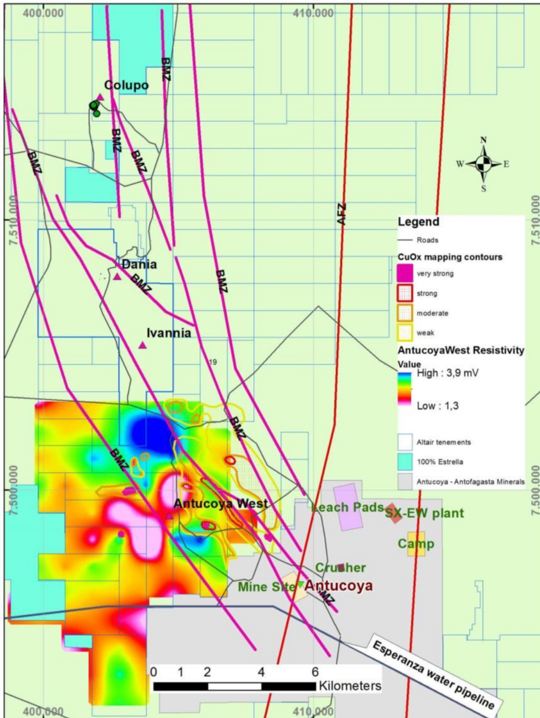
Figure 5: Antucoya West exploration map with contours highlighting prospective zones mapped by Estrella in relation to the anomalous electrical resistivity responses and the BMZ fault zone.
