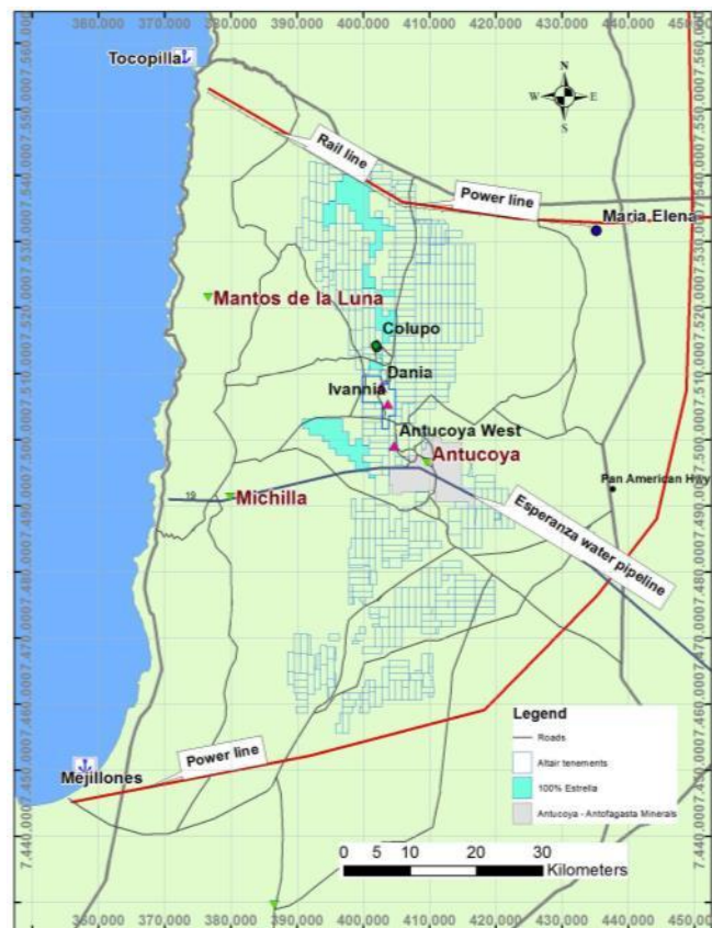
Figure 1: Antucoya West is part of Estrella's Altair Project in Region II northern Chile.
