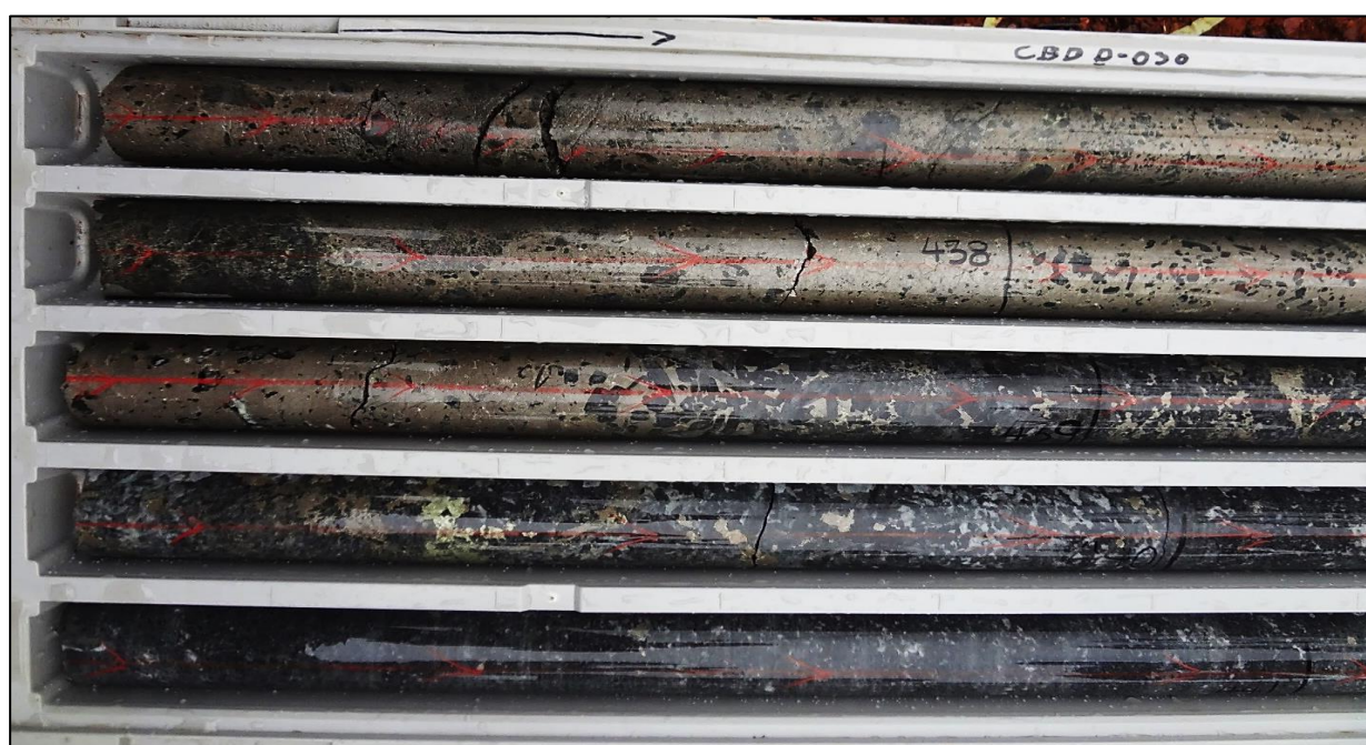
Figure 3. Unique magmatic sulphide textures showing breccia rip up clasts within the massive sulphide, interstitial sulphide/crystal intergrowth at the margin, and chalcopyrite segregation within the crystallised host gabbro. Coarse blebs of matrix sulphide are observed between the crystallising host rock (436.7m-441.1m shown).
