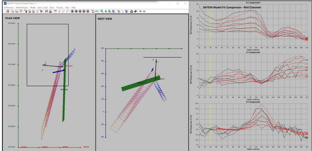
Figure 4. Re-modelling of historical survey data in drill hole DD97CB043 highlighted two local off-hole conductors (blue plates) of moderate conductance and a strong background response that warranted further investigation. Red & purple plates are the original 1997 DHEM models, green is the MLTEM model.
