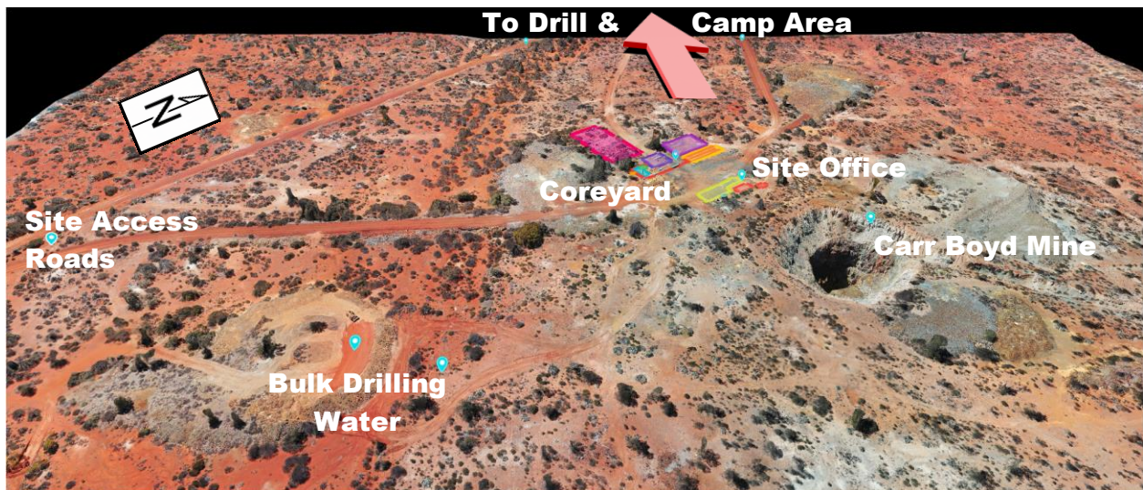
Figure 1. 3D aerial drone survey of the Carr Boyd Mine area showing planned site layout which is currently being established.
