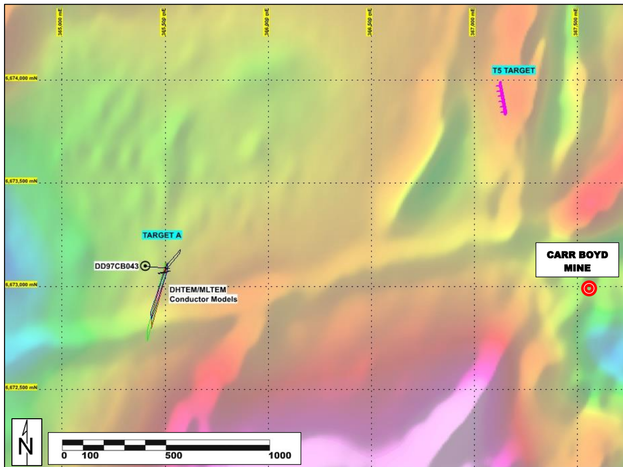
Figure 3. DD97CB043 Drill Hole Location / DHTM-MLTEM Conductor Models over RTP Aeromagnetic Imagery – T5 Location/Conductor AND Carr Boyd Mine are also defined.
