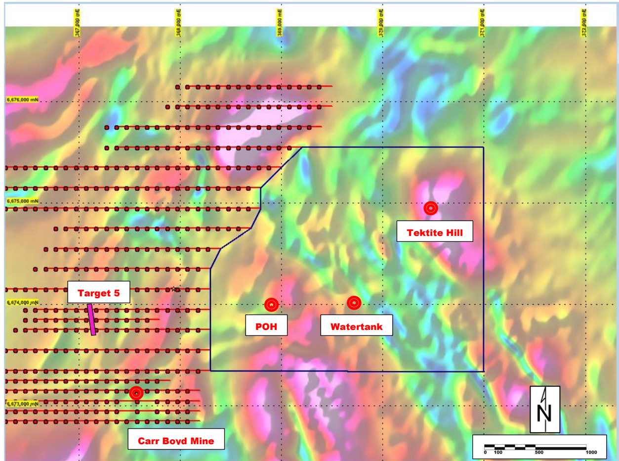
Figure 7. Existing HPMLTEM stations on RTP Aeromagnetic Imagery. T5 and Carr Boyd Mine are located in the west of the area with key regional prospects POH, Watertank and Tektite Hill located to the northeast. The box shows the area of the recent extensional HPMLTEM survey.
