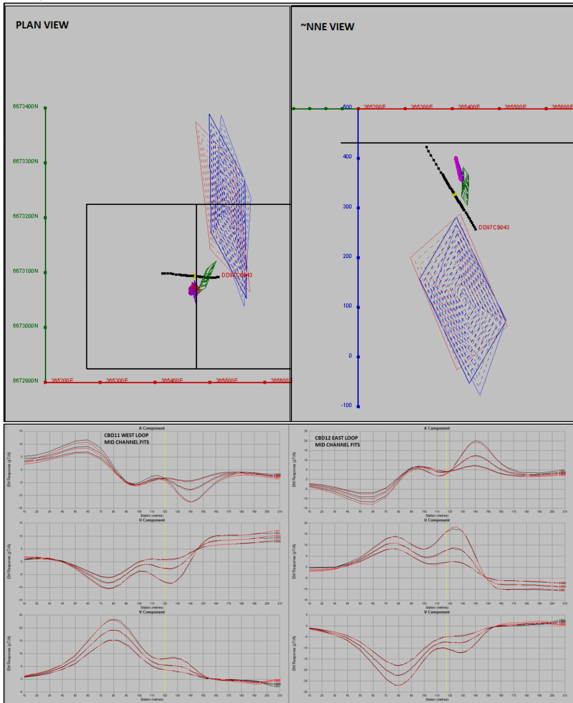
Figure 5. Modelling of new HP DHTeM survey data from resurveying down historical hole DD97CB043 shows different and broader anomalies than the historical survey data shown at Figure 4.
