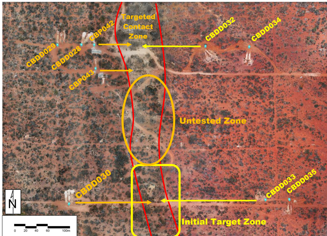
Figure 2. Drone aerial photo of the T5 drill area showing the colour contrast of the targeted ultramafic contact zone between the darker footwall zone (west) and the red iron-rich intrusion (east). The completed drill holes are on the western side of contact and were drilled from the footwall side of the intrusion, the current drill holes are now drilling from the eastern side through the intrusion and back towards the contact zone. Historical holes can still be seen and did not locate this blind nickel sulphide mineralisation as they were drilled to shallow.
