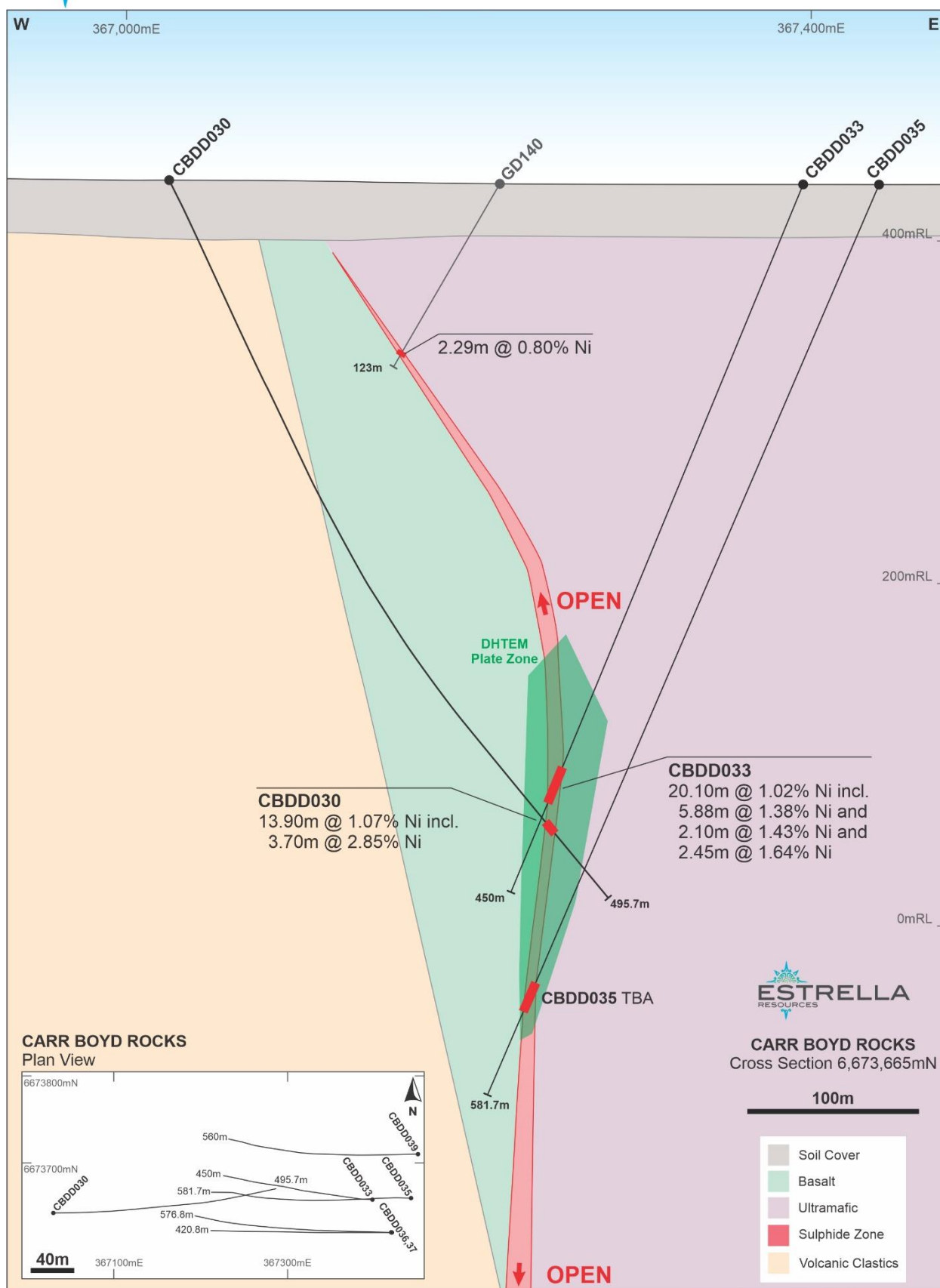
Figure 4. Cross-Section through 6673665mN showing intersection through the sulphide zone and corresponding DHTEM anomaly modelled plate zone. The mineralisation is open up and down the mineralised basal contact zone.
