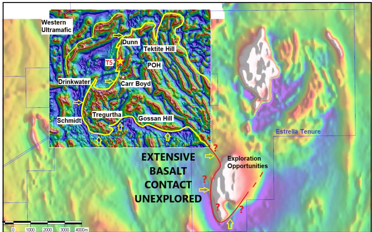
Figure7: Prospect locations along the Carr Boyd Igneous Complex basal contact
