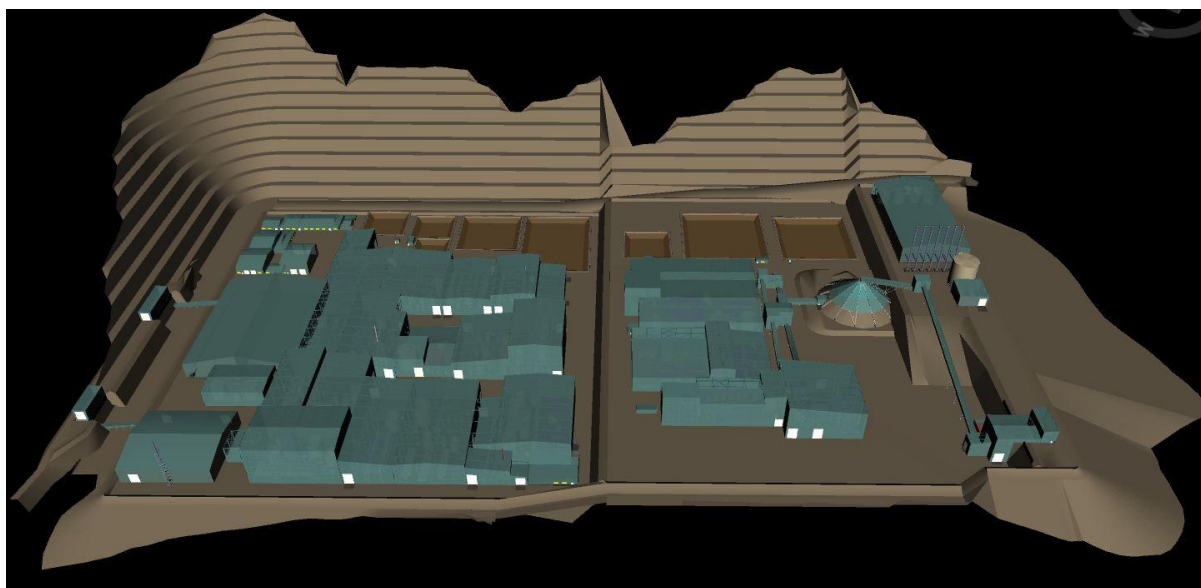
Figure 2. Optimised plant layout with both the Concentrator and Refinery located in a single site. The ROM stockpiles have been removed from the site, and relocated to the mining area where they can be readily accommodated.
