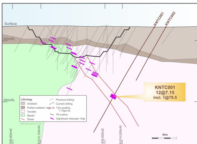
Figure 4: Schematic section of reported holes from Kintore
