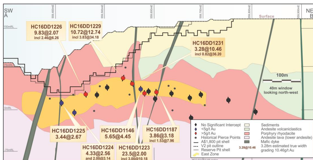
Figure 6: Schematic section of reported drill holes at Mt Carlton
