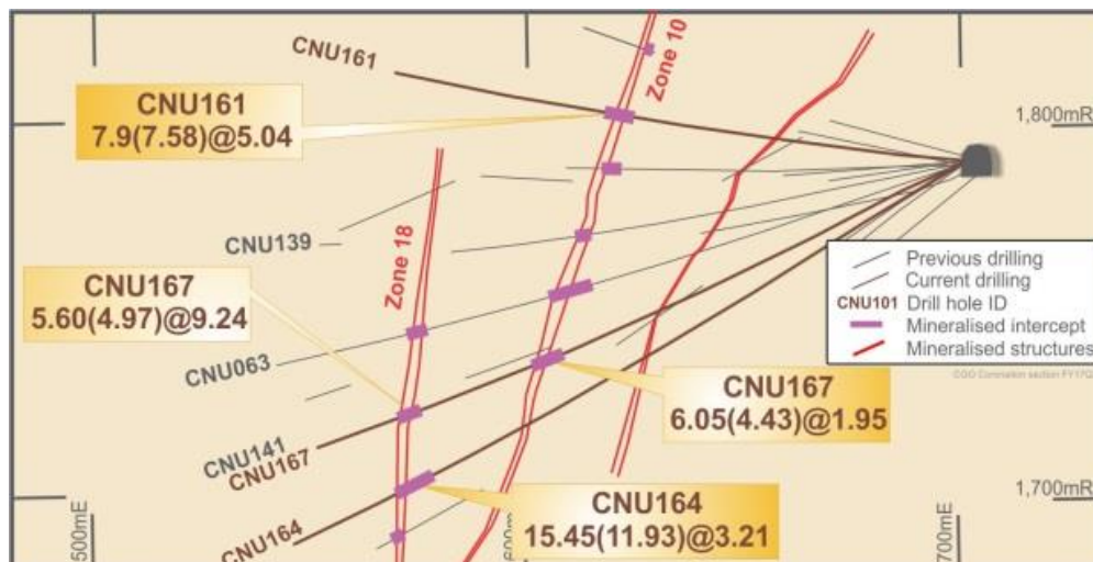
Figure 7: Schematic section of Coronation resource definition drill holes
