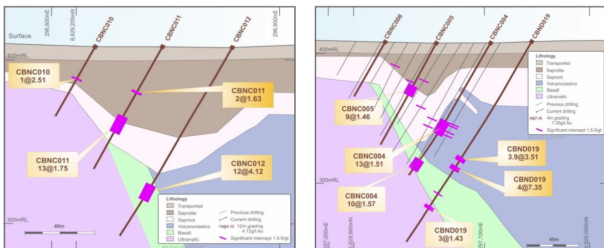
Figure 5: Schematic oblique sections of Carbine North drilling
