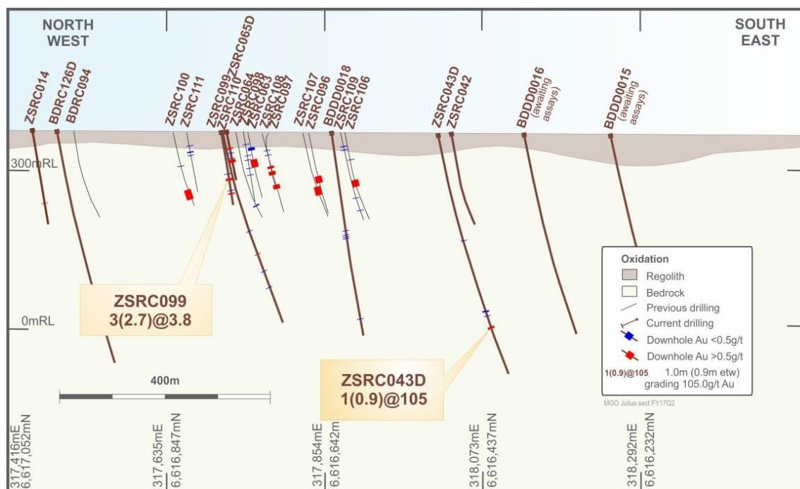
Figure 2: Schematic oblique section of intersections returned from step-out drilling at the Julius prospect
