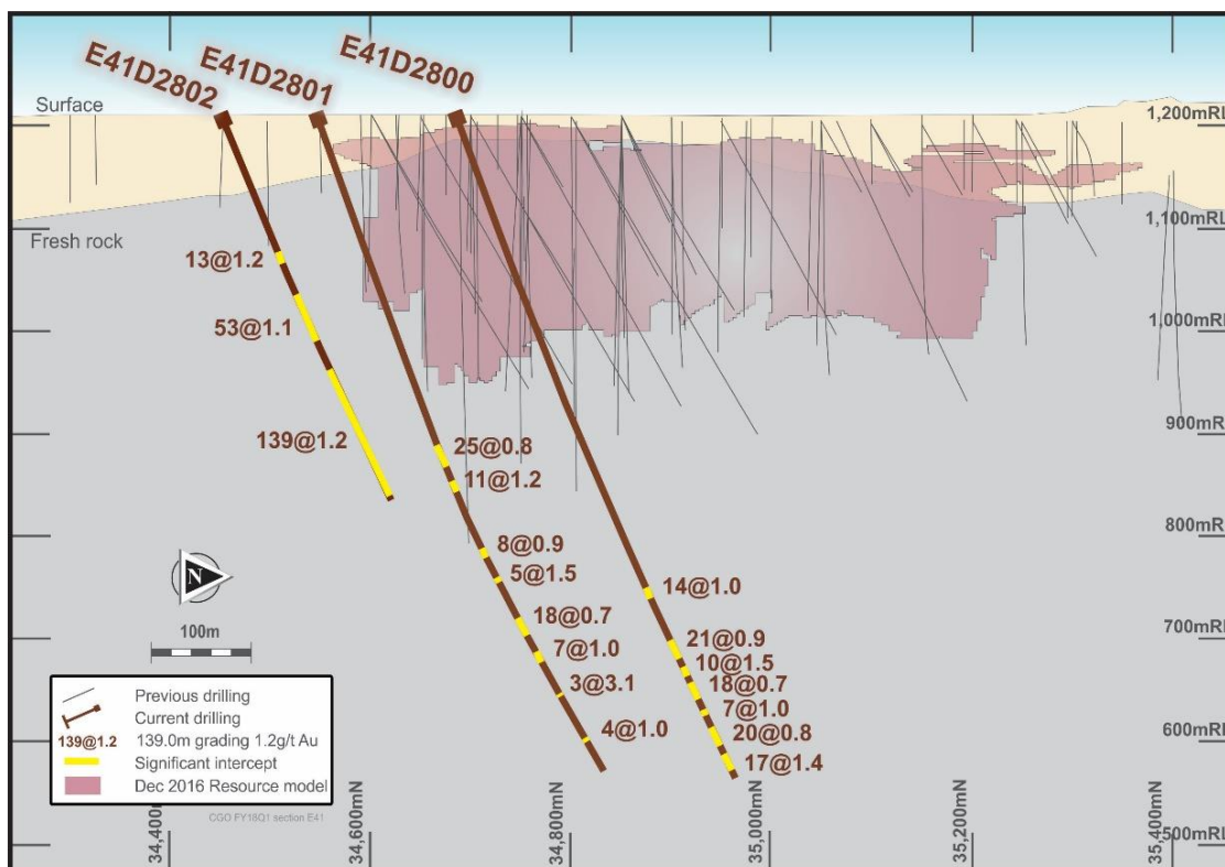
Figure 2: Cross section showing recent drilling E41D2800 - 2801 at E41 Cowal beneath the current resource
