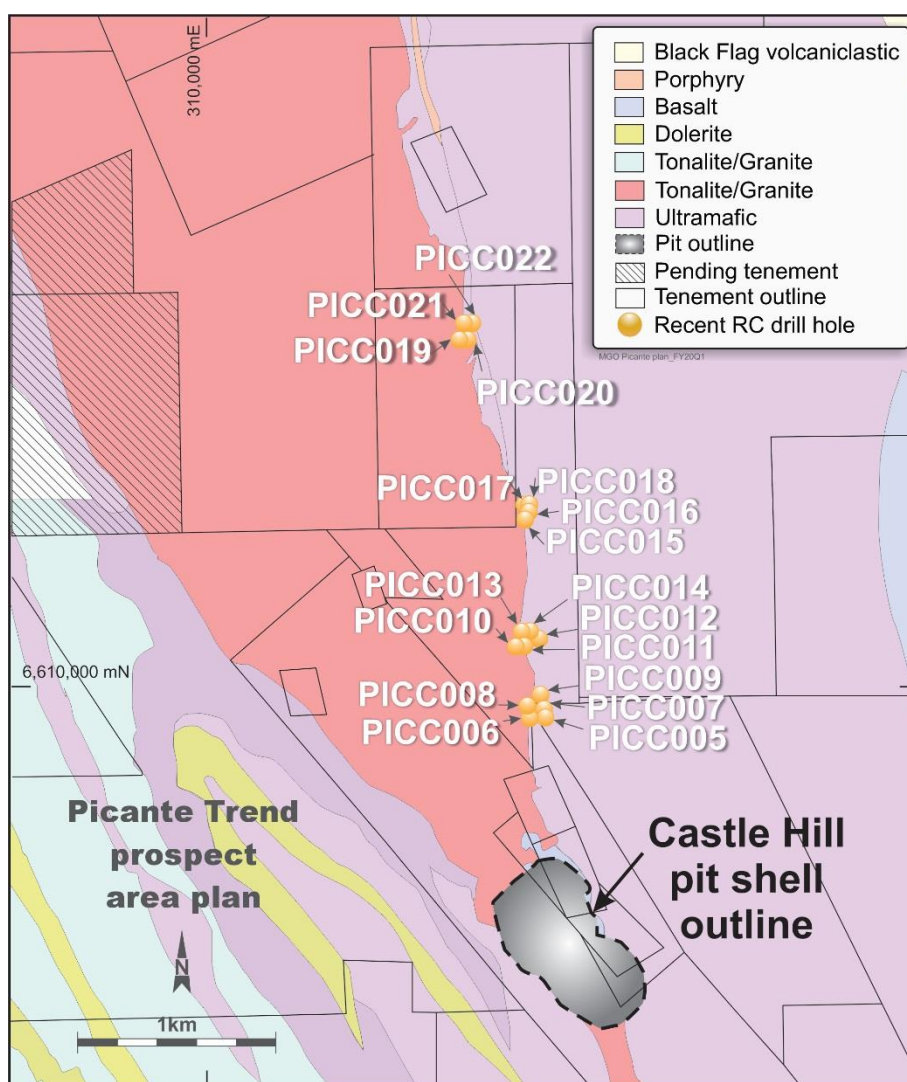
Figure 5: Plan map of the Picante Trend prospect and current drill location
