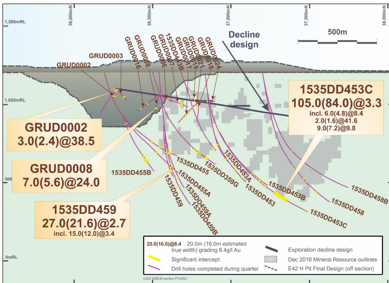
Figure 1: Long projection of the GRE46 structure looking west showing the location of drilling completed during the September quarter
