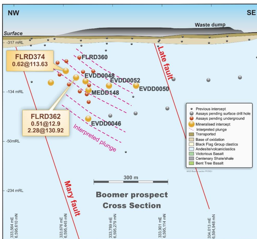
Figure 4: Boomer prospect long section showing location of drilling during the September quarter
