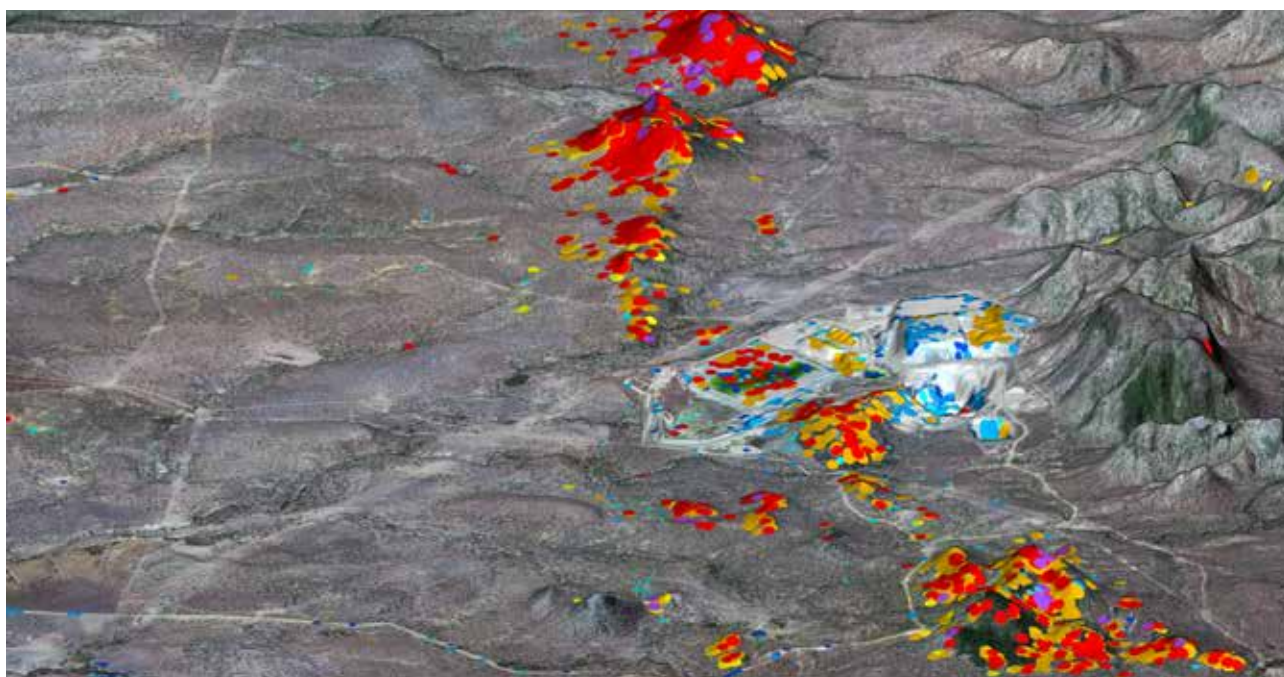
Mineralisation at Mt Carlton developed within magmatic hydrothermal centres. We identify “hot spots” as accumulations of low pH clay
