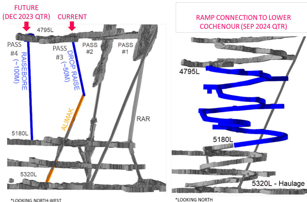
Figure 1: De-risking the Cochenour pass system by creating multiple options to move material to the haulage level via two new ore passes and a ramp alternative
