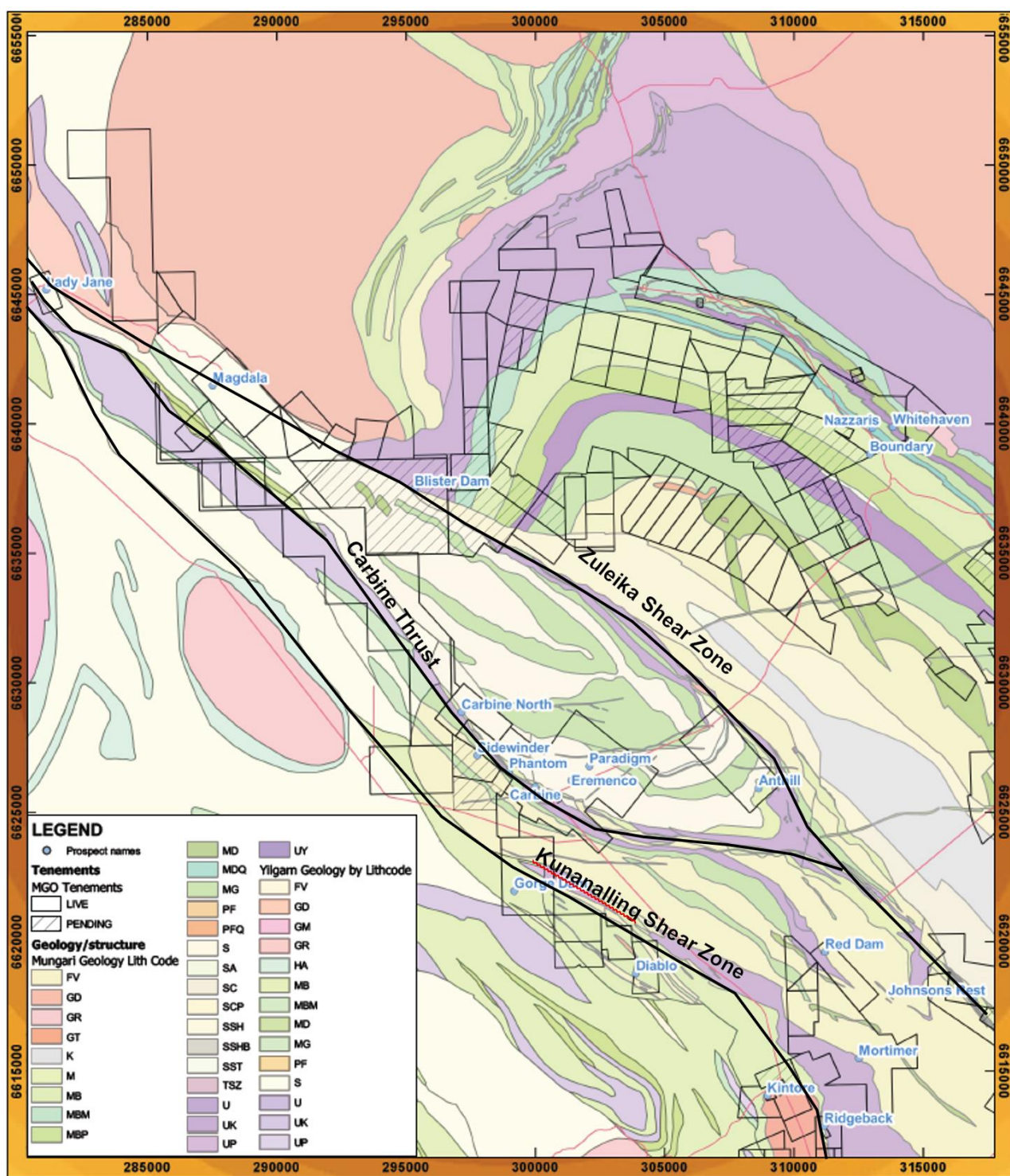
Figure 24: The Carbine Zuleika project area sub-surface Geology.
