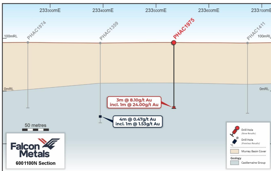
Figure 3 Cross Section showing high-grade result in PHAC1975
