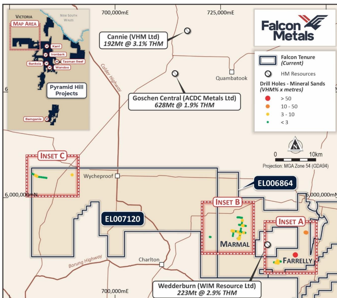
Figure 6 Location map of the initial phase of mineral sands drilling at Pyramid Hill
