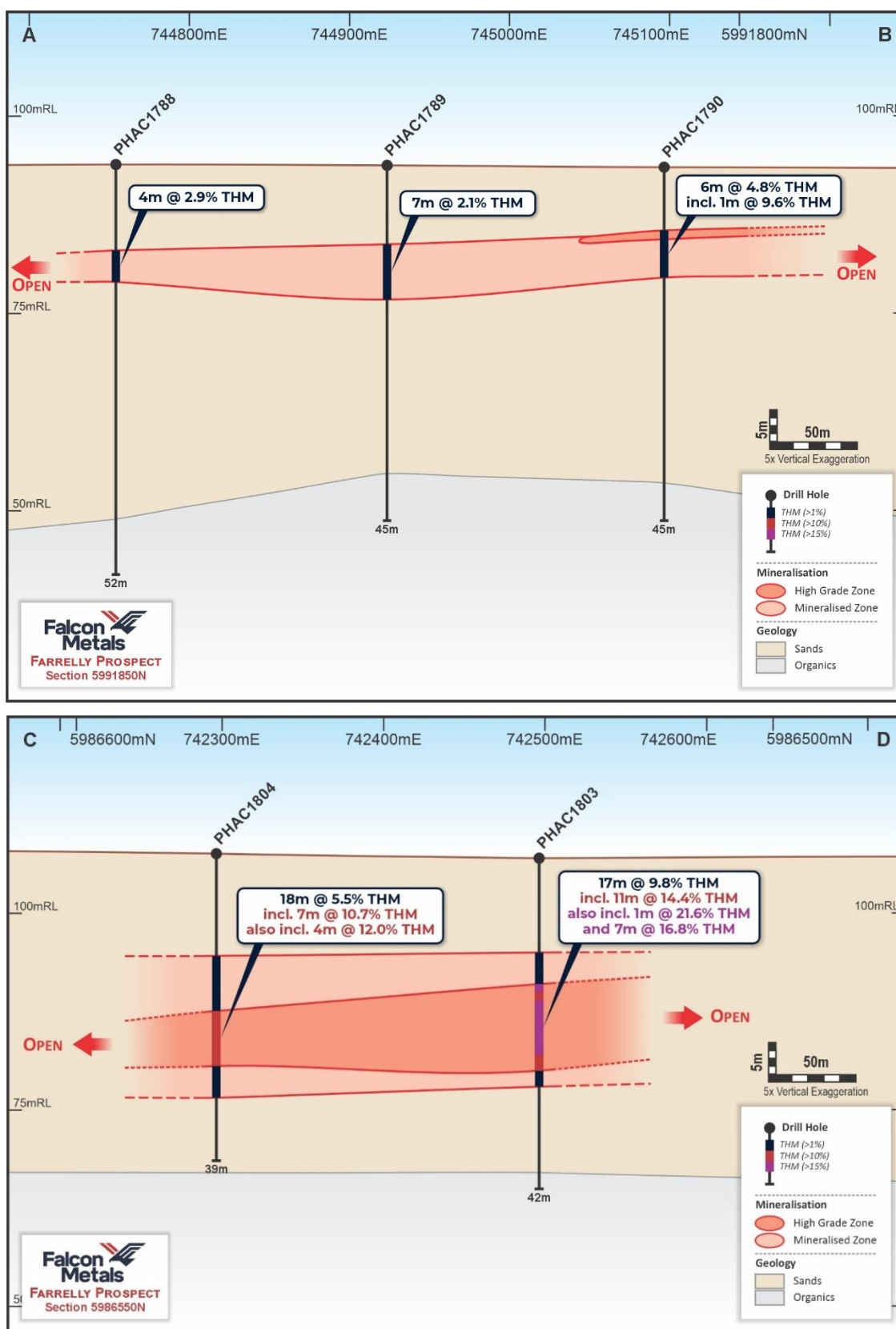
Figure 8 Cross-sections A-B and C-D through the Farrelly Prospect showing holes with results received
