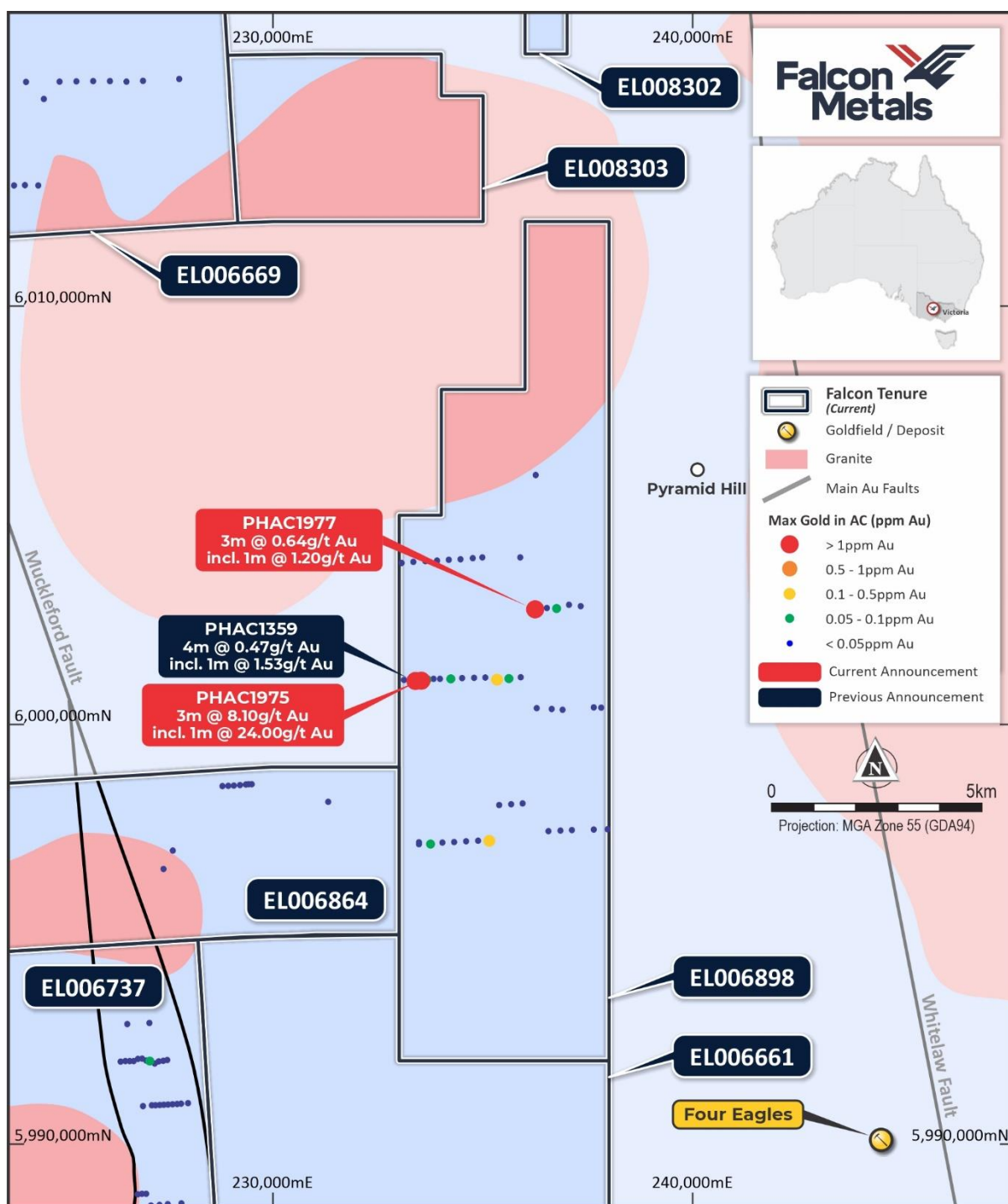
Figure 2 Location map of Whitelaw Fault drilling with maximum gold
