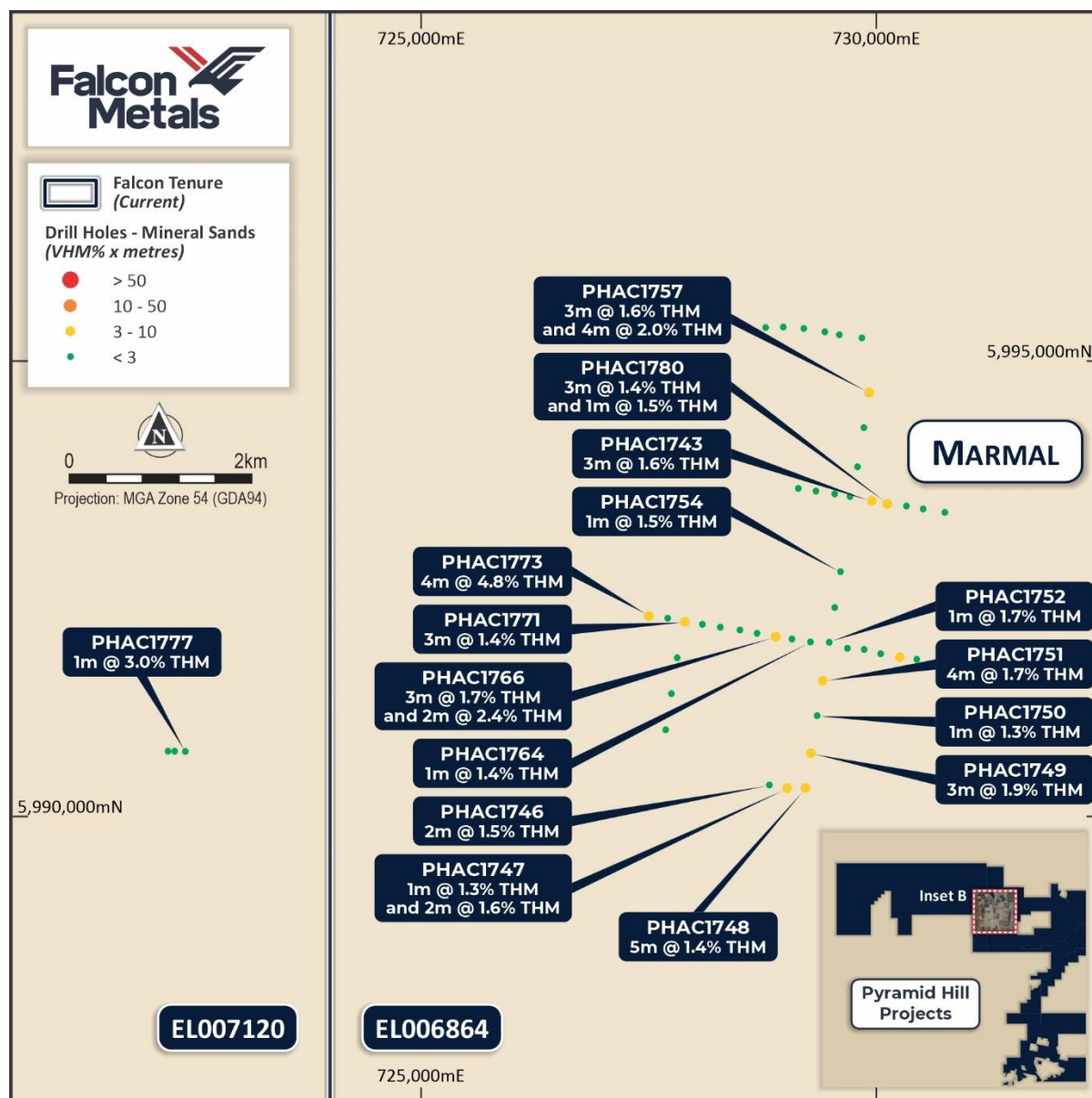
Figure 9 Plan map of the Marmal Prospect
