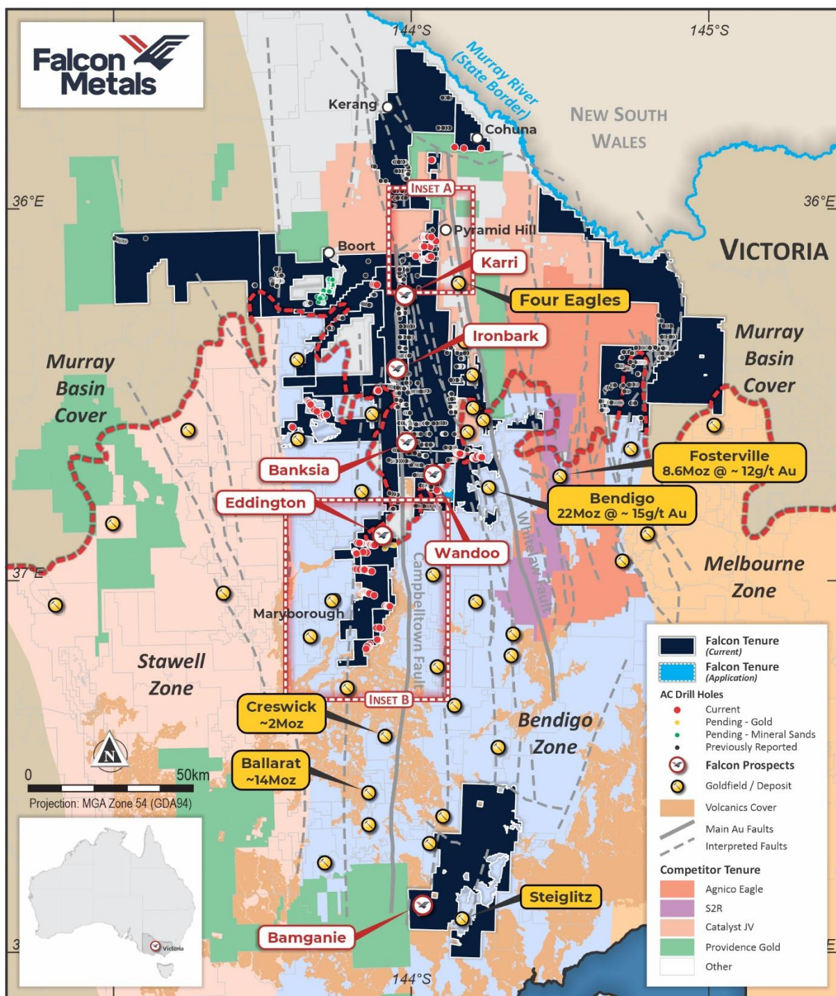
Figure 1 Plan map showing the locations of Falcon's key gold prospects and drilling status
