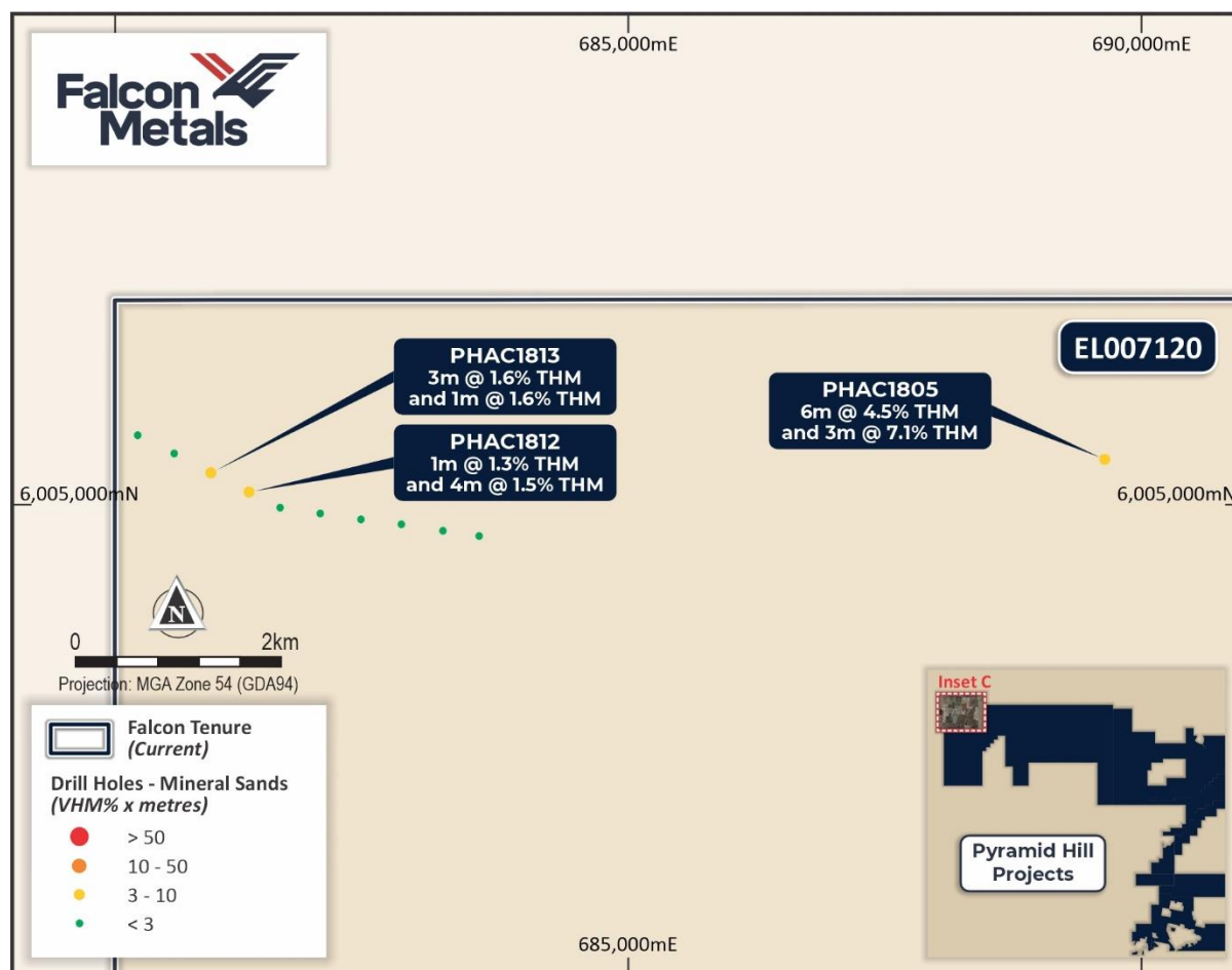
Figure 10 Plan map of the drilling in the northwest of EL007120
