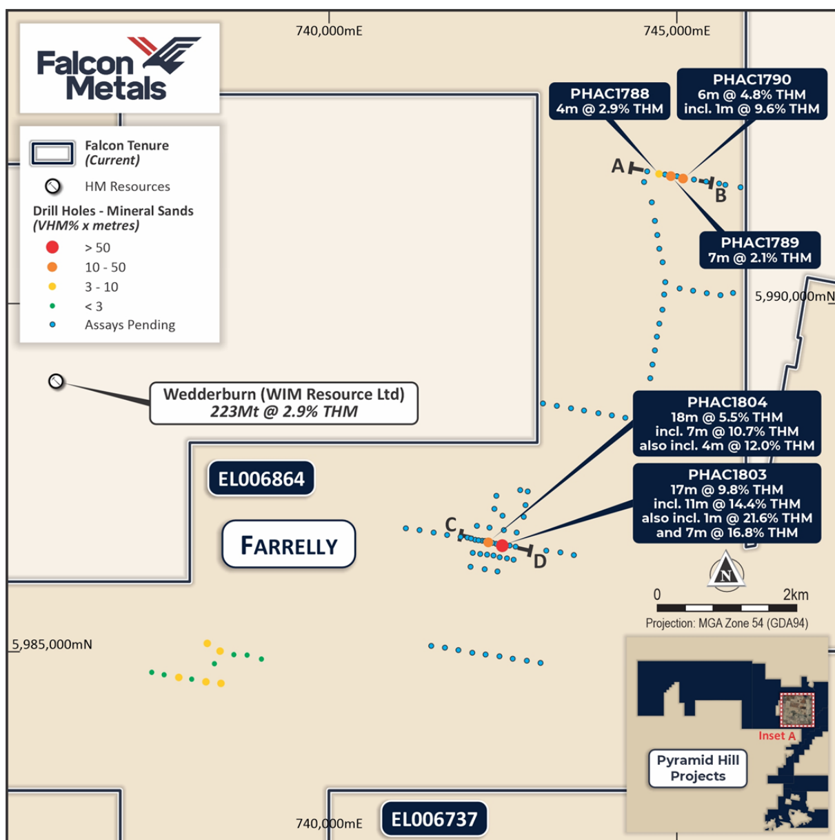
Figure 7 Location of the Farrelly Prospect showing results received and recently completed follow-up drilling awaiting assays
