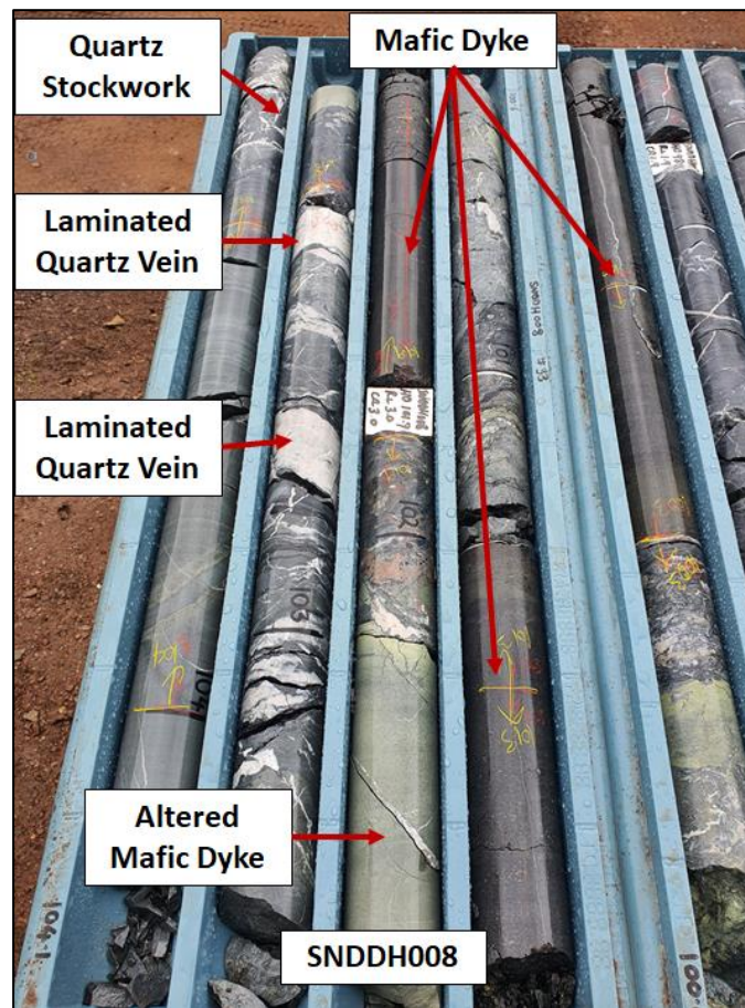
Figure 2: Mineralised quartz-veins intimately associated with mafic intrusions.
