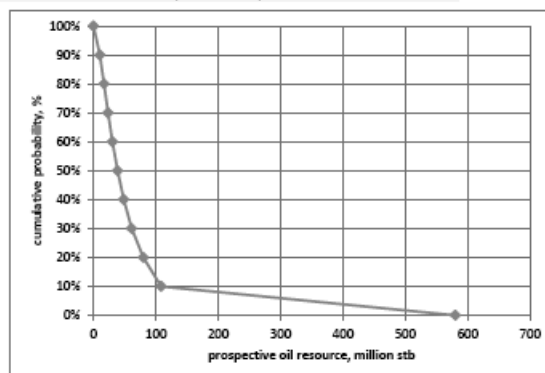
Figure 8 Betioky prospect prospective oil resource distribution
