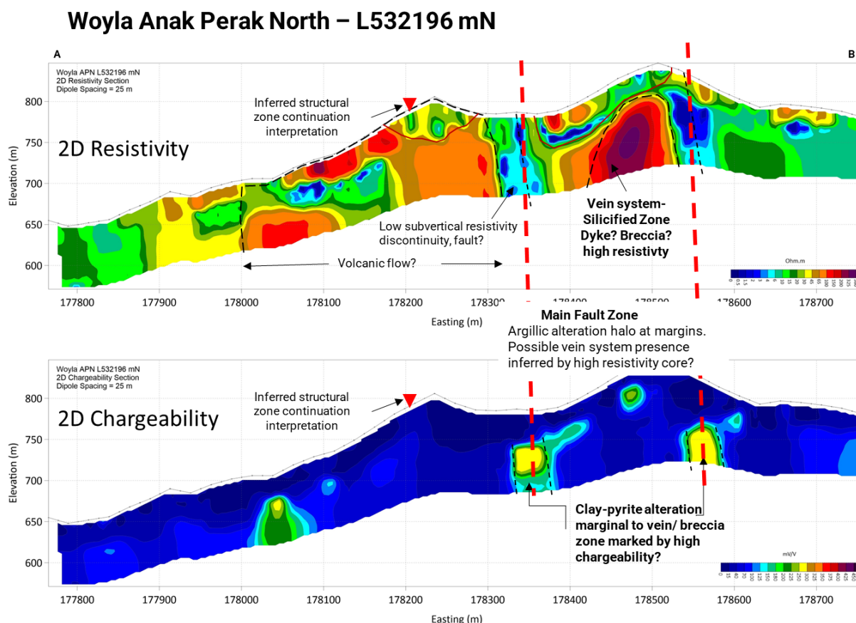
Figure 5: Image shows interpretation and modeling of IP survey data. Infers an approximate 100m wide structural zone with central high resistivity anomaly and high chargeability margins. This signature is consistent with the presence of an epithermal quartz vein/breccia with development of argillic alteration in adjacent wallrock.
