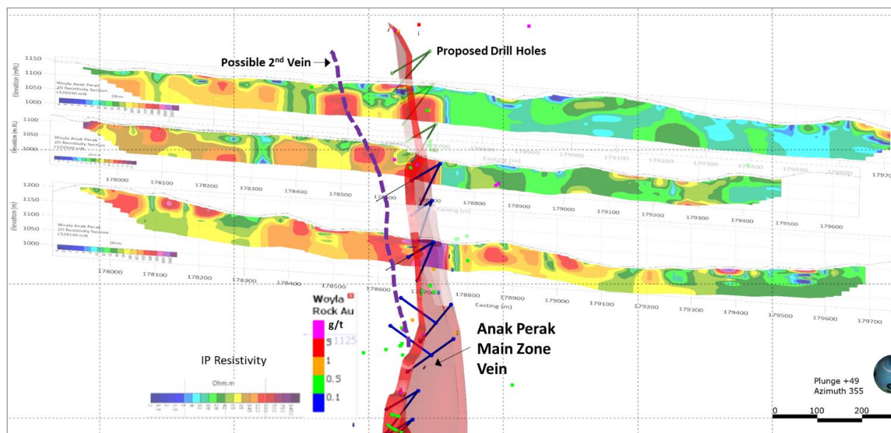
Figure 3: Map showing a 3D image of the Anak Perak Main Zone area. The Anak Perak Main Zone vein as previously mapped on surface is indicated by completed lines of IP survey. The presence of a possible secondary vein to the west is indicated.
