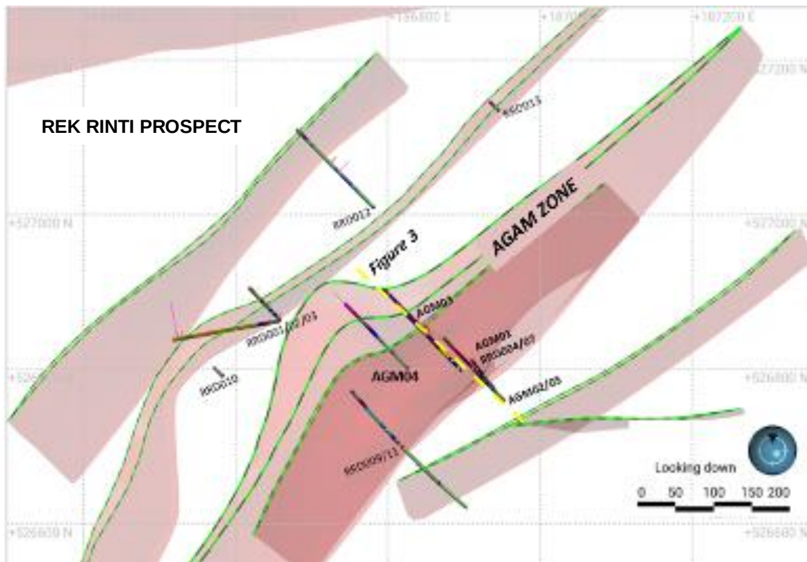
Figure 1: Plan map showing the interpreted surface extent of the Agam Zone veins at Rek Rinti. The location of completed Phase 1 and current Phase 2 drillholes including AGM004 are indicated. The interpreted dilation/flexure of the zone is shown as is the location of the drill section shown in Figure 3.
