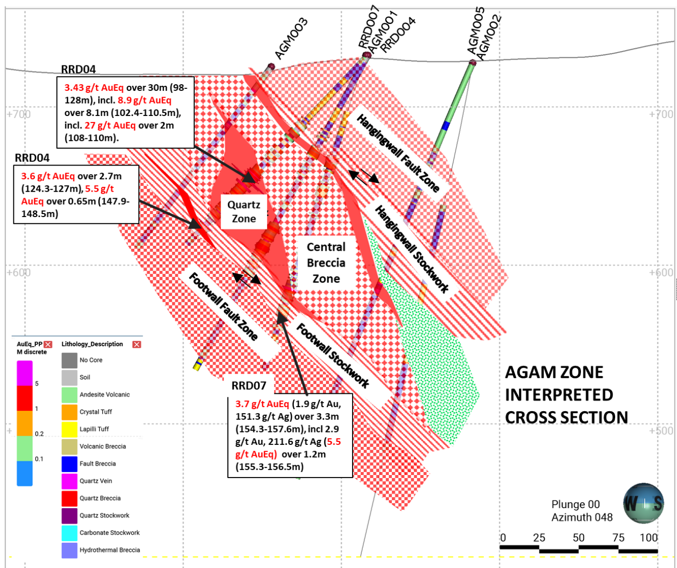
Figure 3: Interpretive cross section of the first completed drill section across the Agam Zone. The zone is characterised by hangingwall and footwall faults at zone boundary with outer quartz stock vein zones and central zone of massive quartz and quartz breccia. The best developed (and highest grade) mineralization occurs within the central breccia zone and zones of massive quartz contained therein. The cross section will be revised as more holes are drilled. Assays are pending for Phase 2 AGM drill holes.
