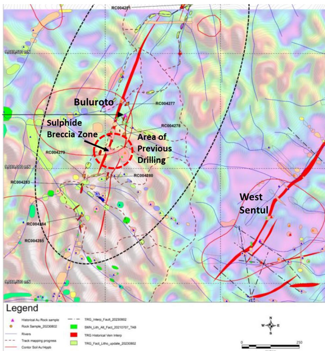
Figure 7: Area of mapping over the Buluroto vein system. In contrast to the Sentul vein system Buluroto occurs adjacent to a broad area of high magnetics. The zone of Cu-enriched sulphide breccia intersected by previous drilling occurs on the margin of a high-magnetic zone suggesting it's development could be porphyry related.
