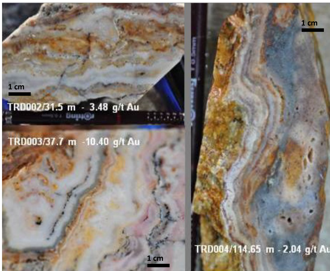
Figure 5: Core specimens of drillholes in the West Sentul vein system showing examples of crustiform-colloform quartz- sulphide textures that occur. These are characteristic of ginguro-type bands that are often associated with high-grades of gold-silver in such vein systems. The gold grades indicated are recorded in historical assay reports. While the Company has confirmed the presence of such textures it has not conducted any additional core sampling to confirm reported grades.
