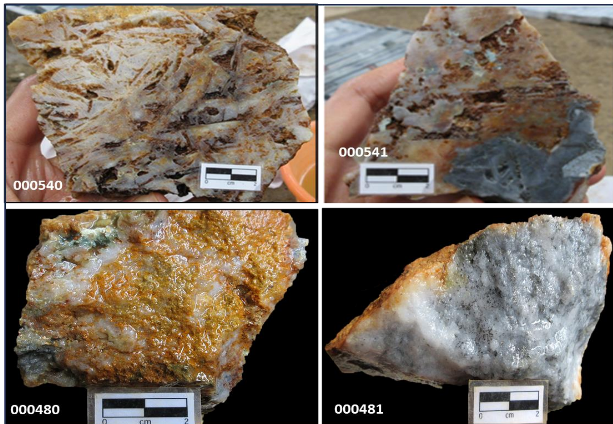
Figure 3: Grab samples of Aloe Rek vein material in artisanal mining pits; 000540) bladed quartz vein sample taken at 20m depth from 3-5m wide vein, assay of 14.9 g/t Au, 22.1 g/t Ag; 000541) taken at 20m depth from an artisanal mining shaft. Abundant arsenopyrite in lower right. Assay of 9.1 g/t Au, 20.5 g/t Ag. The samples also contain high antimony (Sb). Refer to Table 1. 000480) oxidized, crystalline quartz from 60m depth. assay 76 g/t Au, 78 g/t Ag, 000481) crystalline quartz with abundant fine-grained arsenopyrite, assay 23.8 g/t Au, 30 g/t Ag.
