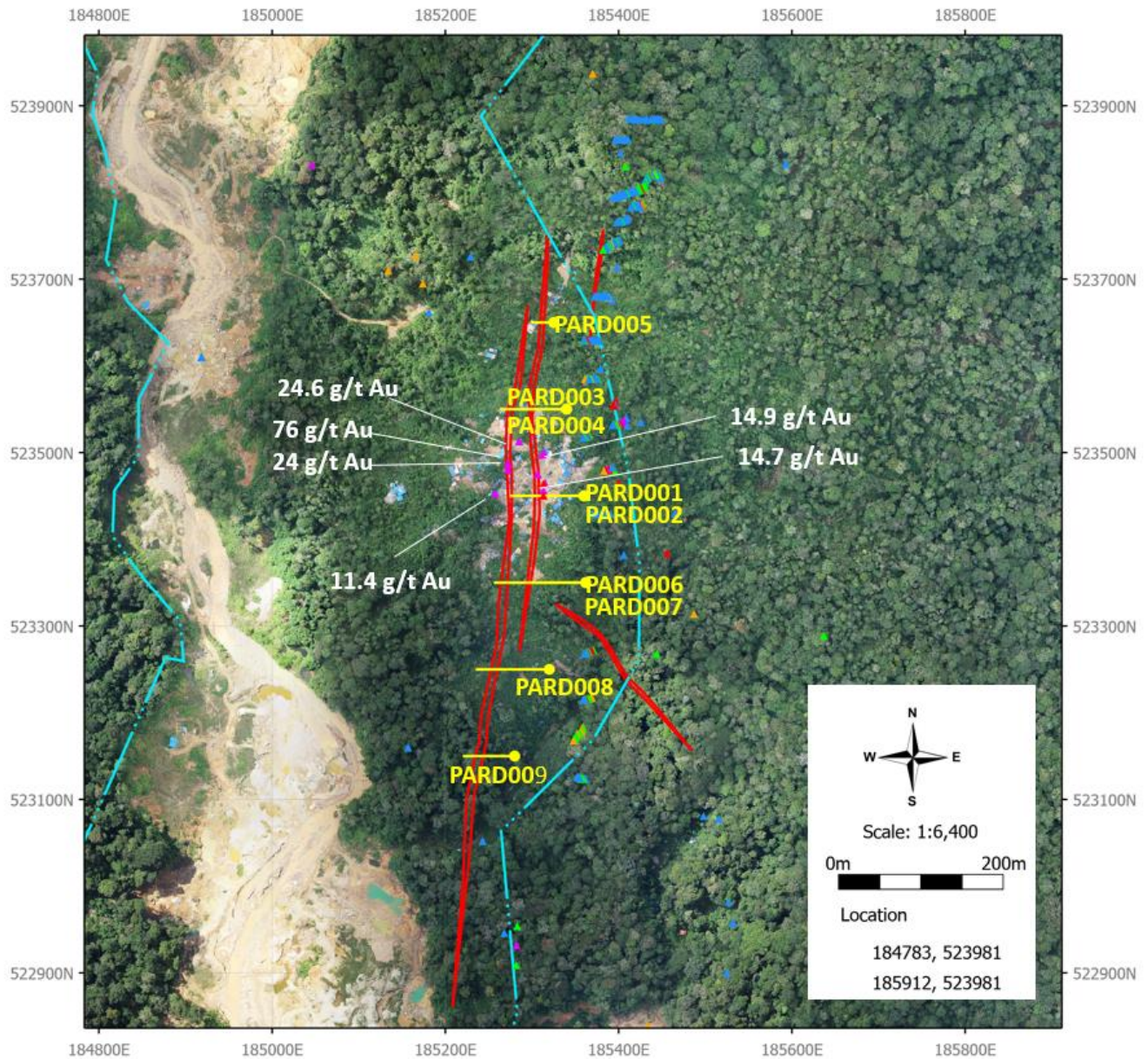
Figure 4: Satellite image of the Aloe Rek prospect area showing the locations of proposed drill holes and Au assays from collected vein samples. Refer to Table 1.
