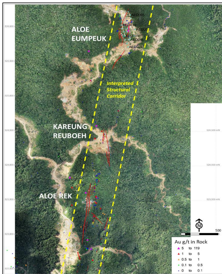
Figure 1: Plan map showing the interpreted extent and orientation of quartz veins within the interpreted structural corridor extending south from the Aloe Eumpeuk prospect area to Aloe Rek. Reported assays from the recently discovered Kareung Reuboeu veins confirm the continuation of the vein system and also the presence of high-grade Au-Ag mineralisation. See Figure 2 and ASX release of 26 May 2023 for additional sample assay information. Coordinate datum is WGS84 Zone 47N.
