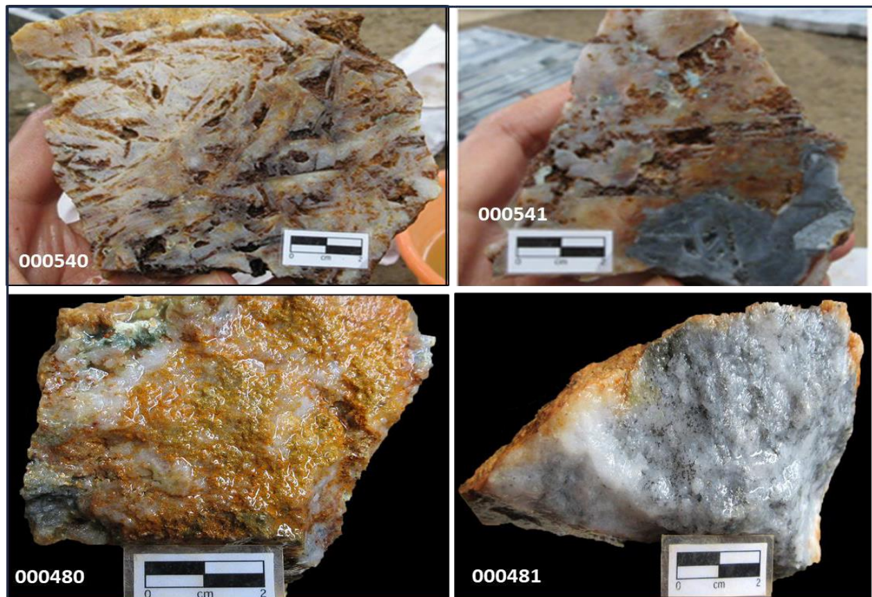
Figure 3: Grab samples of Aloe Rek vein material in artisanal mining pits; 000540) bladed quartz vein sample taken at 20m depth from 3-5m wide vein, assay of 14.9 g/t Au, 22.1 g/t Ag; 000541) taken at 20m depth from an artisanal mining shaft. Abundant arsenopyrite in lower right. Assay of 9.1 g/t Au, 20.5 g/t Ag. The samples also contain high antimony (Sb). Refer to Table 1. 000480) oxidized, crystalline quartz from 60m depth. assay 76 g/t Au, 78 g/t Ag, 000481) crystalline quartz with abundant fine-grained arsenopyrite, assay 23.8 g/t Au, 30 g/t Ag.
