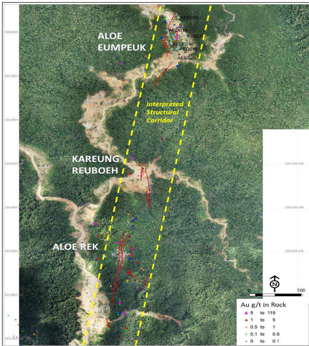
Figure 1: Plan map showing the interpreted extent and orientation of quartz veins within the interpreted structural corridor extending south from the Aloe Eumpeuk prospect area to Aloe Rek. Reported assays from the recently discovered Kareung Reuboeu veins confirm the continuation of the vein system and also the presence of high-grade Au-Ag mineralisation. See Figure 2 and ASX release of 26 May 2023 for additional sample assay information. Coordinate datum is WGS84 Zone 47N.
