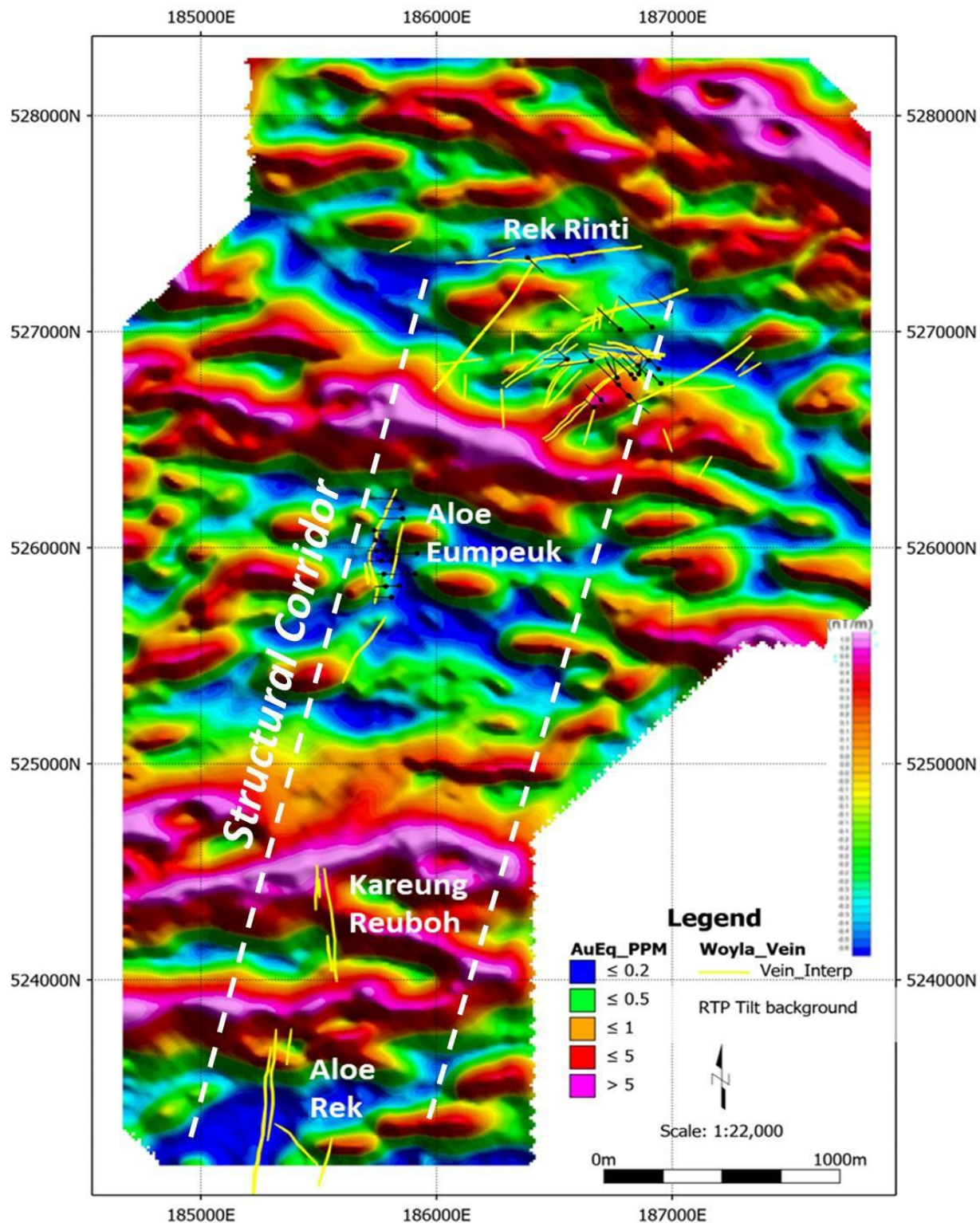
Figure 2: Interpreted RTP tile-filtered image from the UAV magnetic survey at Woyla, Image shows the prominent near East-West trending high magnetics linears and series of North-South trending quartz veins. The image shows that the Aloe Rek veins occur within an area of strong low magnetics inferring it is also an area of intense argillic alteration.
