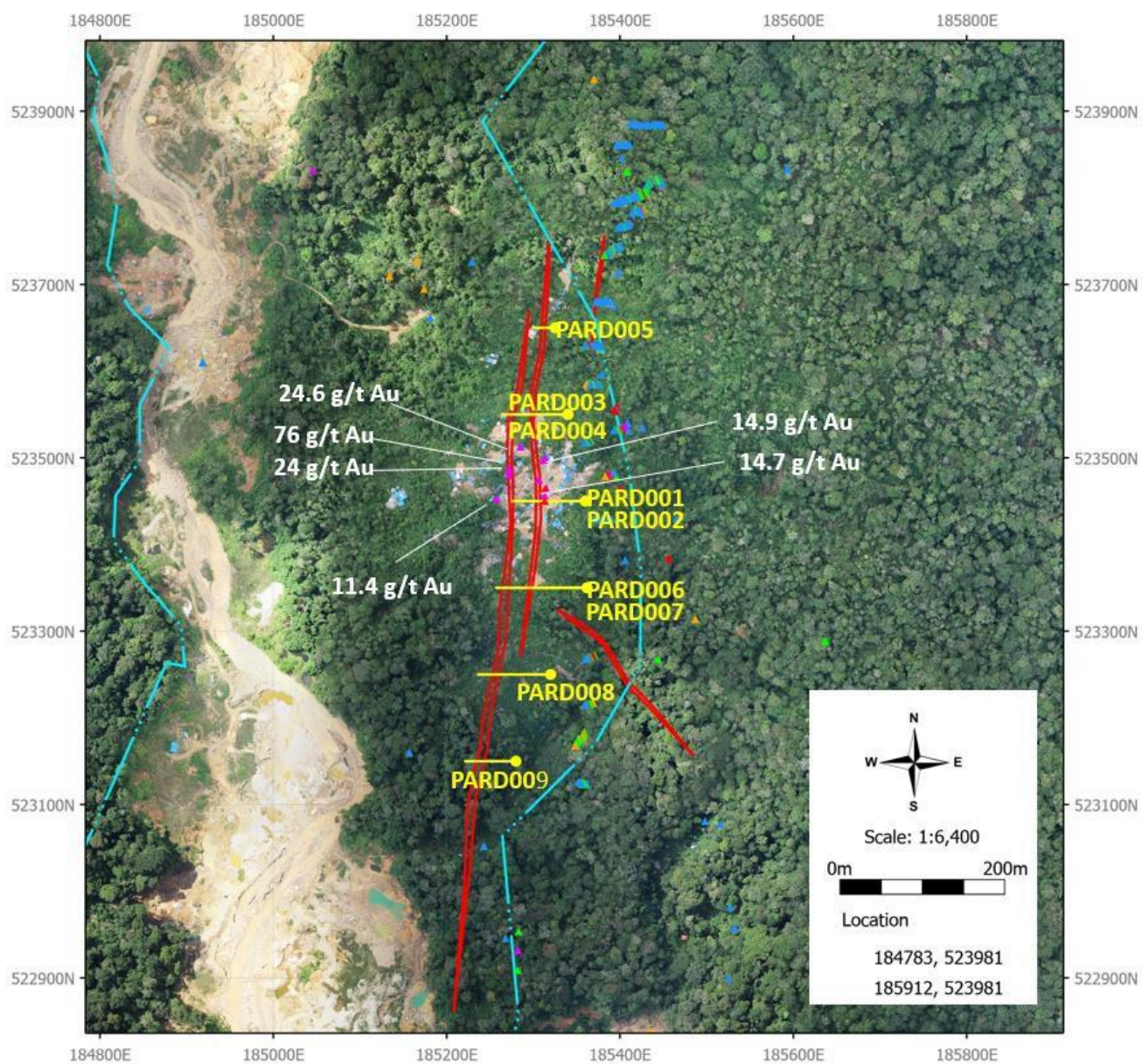
Figure 4: Satellite image of the Aloe Rek prospect area showing the locations of proposed drill holes and Au assays from collected vein samples. Refer to Table 1.
