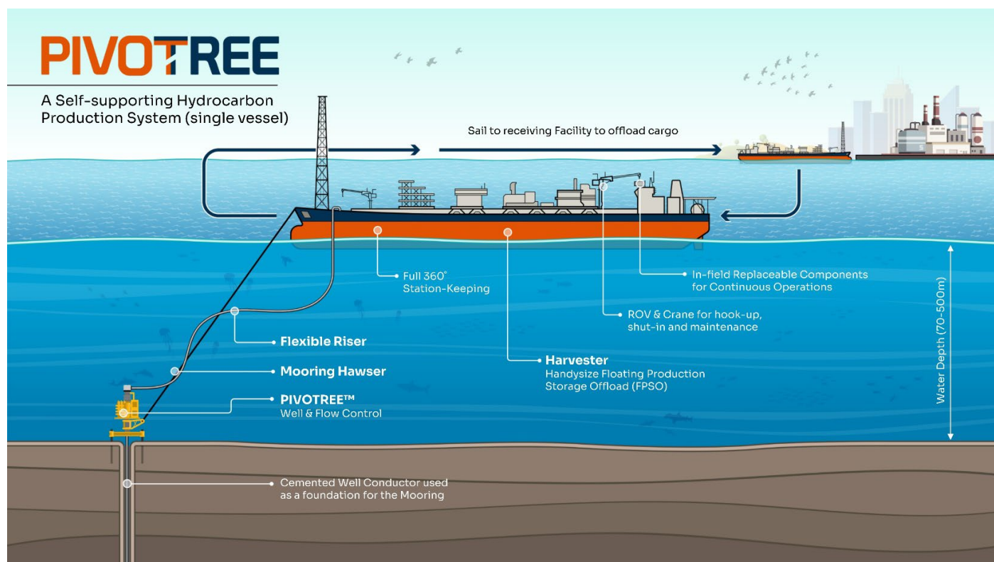
Diagramme of Pivotree development and production concept.
