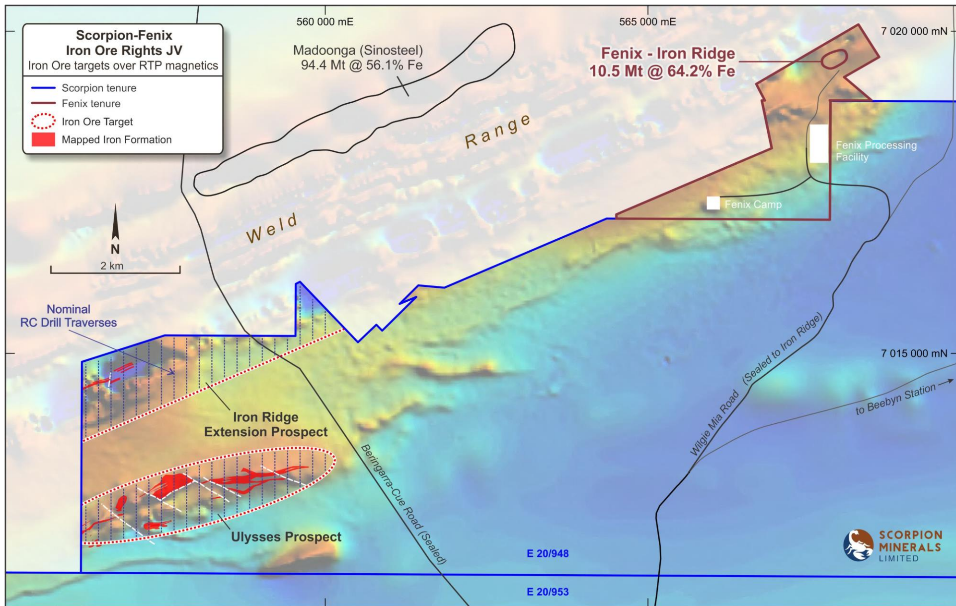
Figure 3 – Weld Range Iron ore targets showing nominal 200m-spaced RC drilling traverses at “Iron Ridge Extension” and “Ulysses” Prospects
