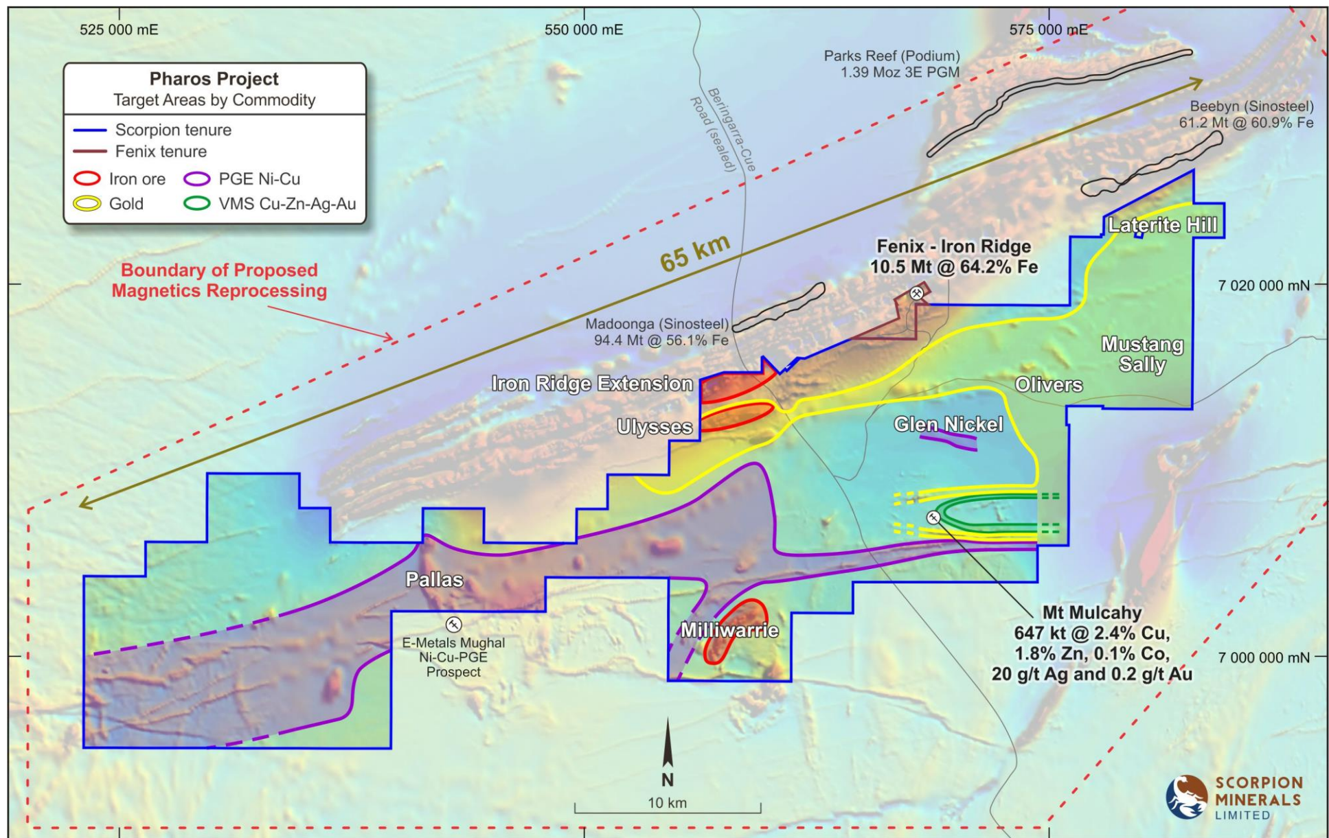
Figure 2 – Area of Reprocessed Open File/Multi Client Magnetics and commodity Targets - Pharos
