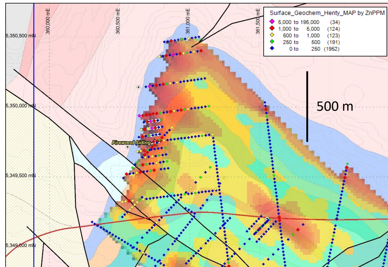
Firewood Siding prospect area interpreted geology with bedrock/C-Horizon wacker sampling grid Zn distribution.
