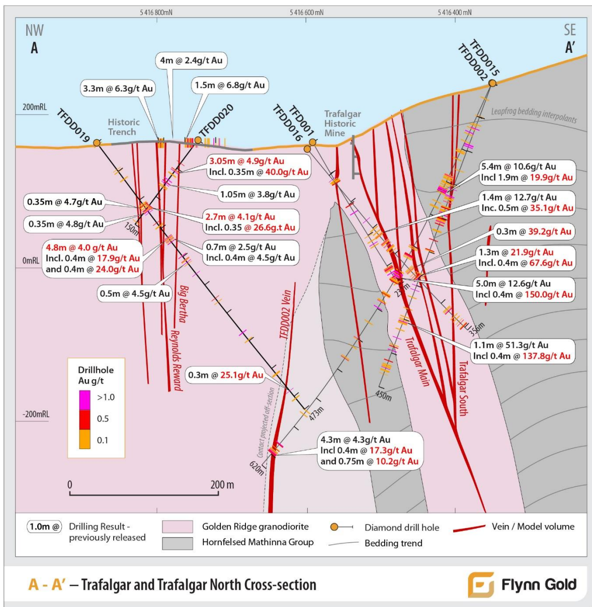
Figure 4 – Trafalgar and Trafalgar North Prospects: Cross-section A-A' (see Figure 2 for location) looking ENE with drilling highlights.
